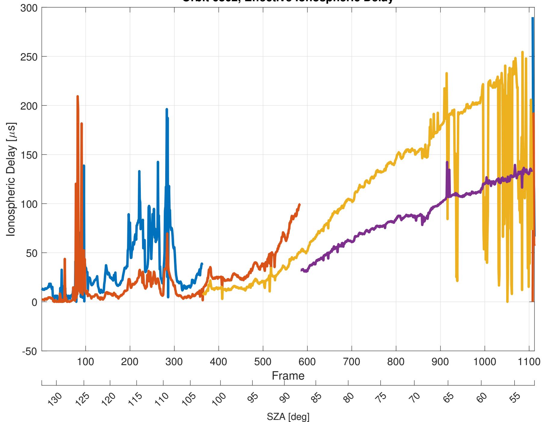
Orbit 6862, Effective Ionospheric Delay
