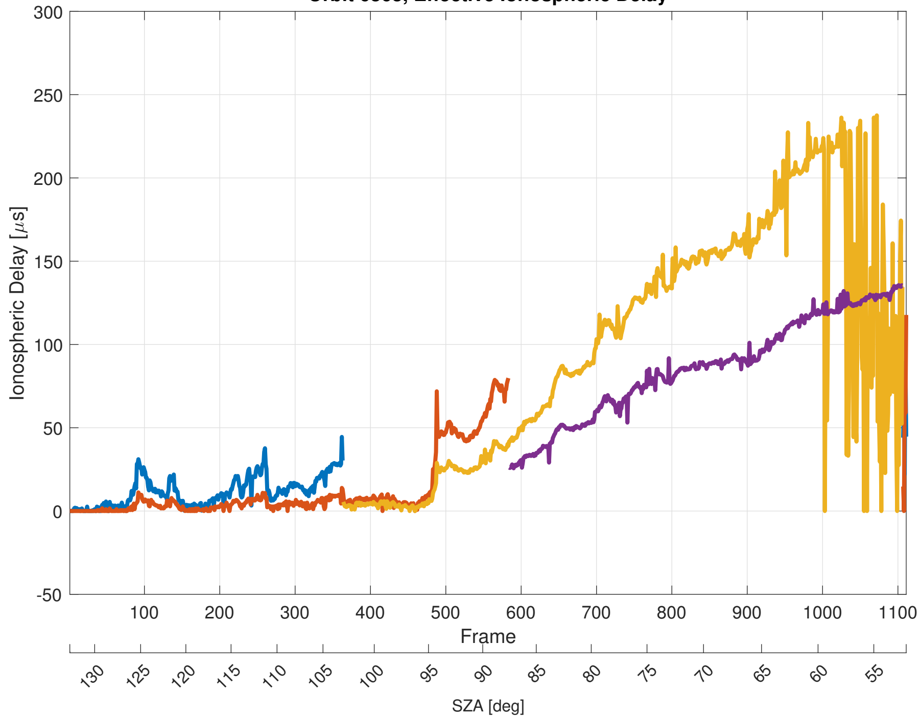
Orbit 6863, Effective Ionospheric Delay
