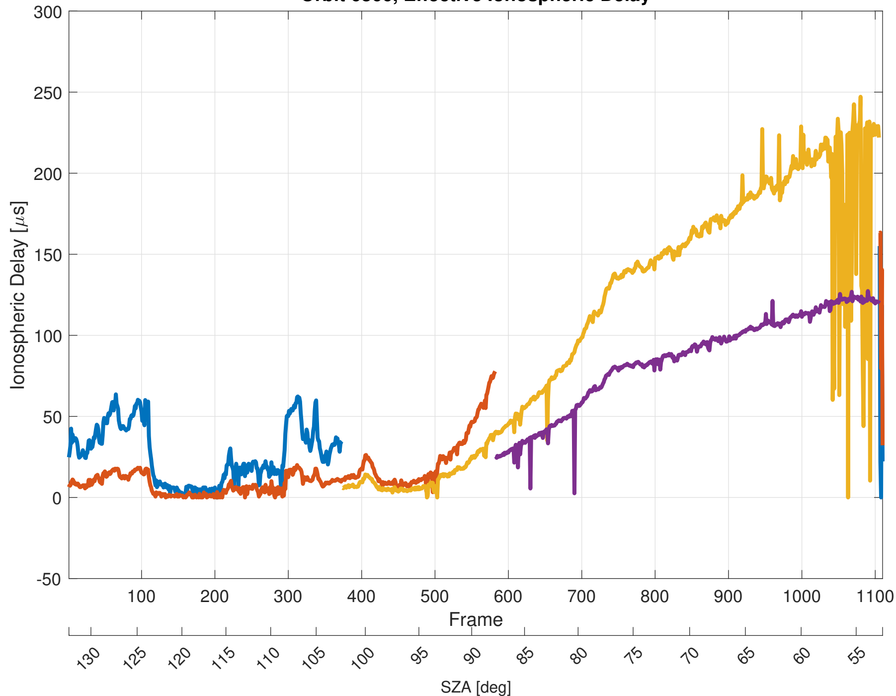
Orbit 6866, Effective Ionospheric Delay
