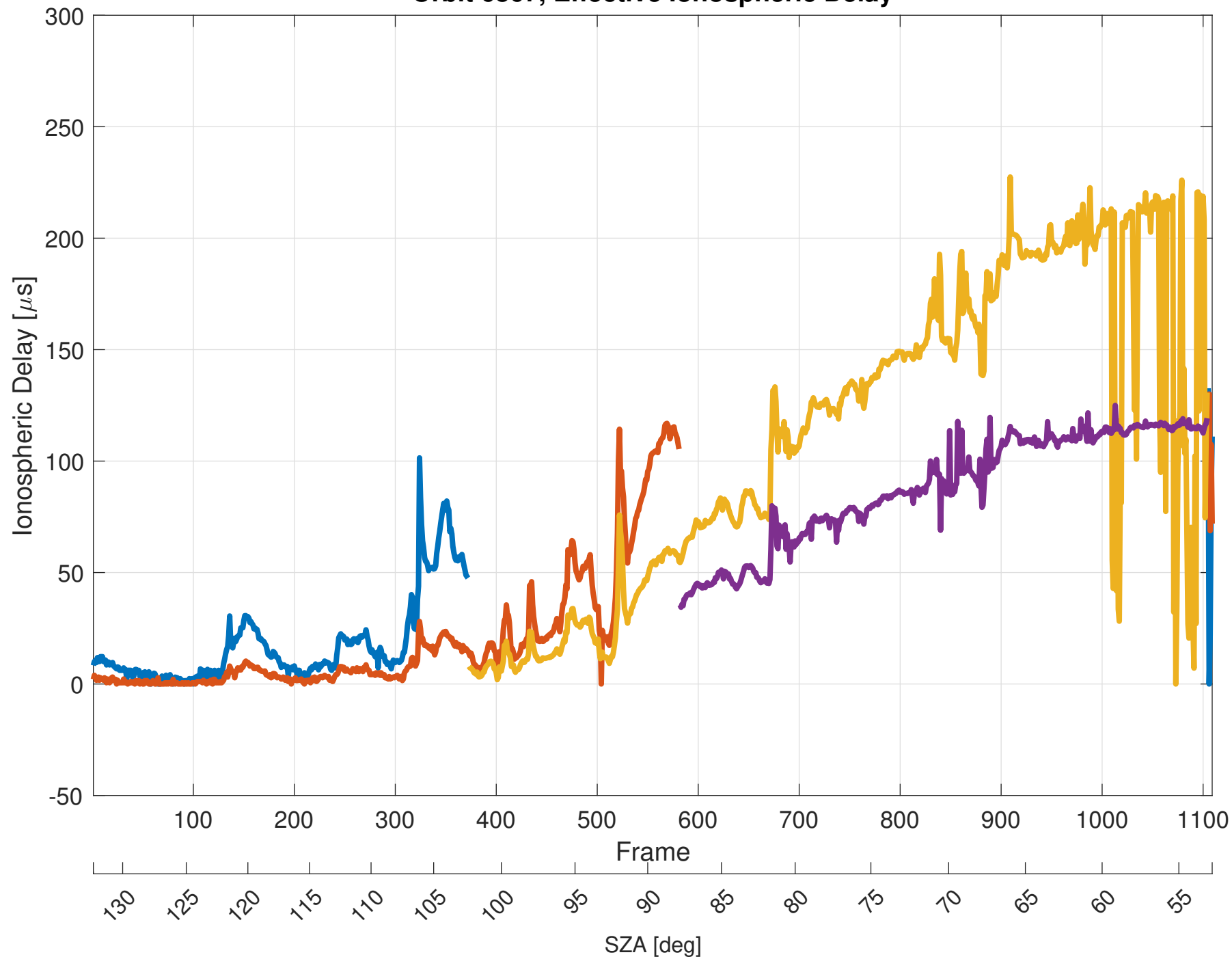
Orbit 6867, Effective Ionospheric Delay
