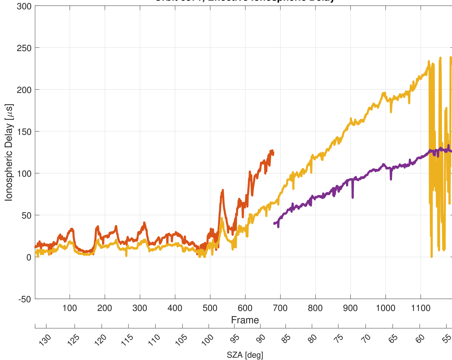
Orbit 6871, Effective Ionospheric Delay
