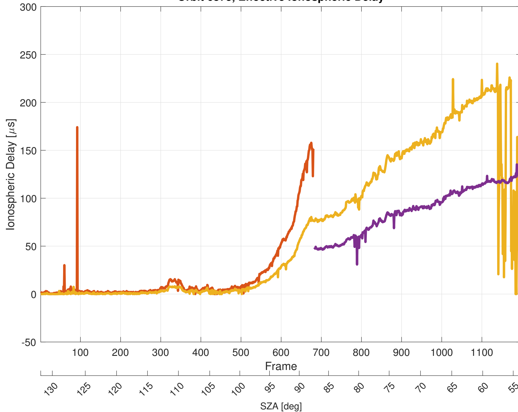
Orbit 6873, Effective Ionospheric Delay
