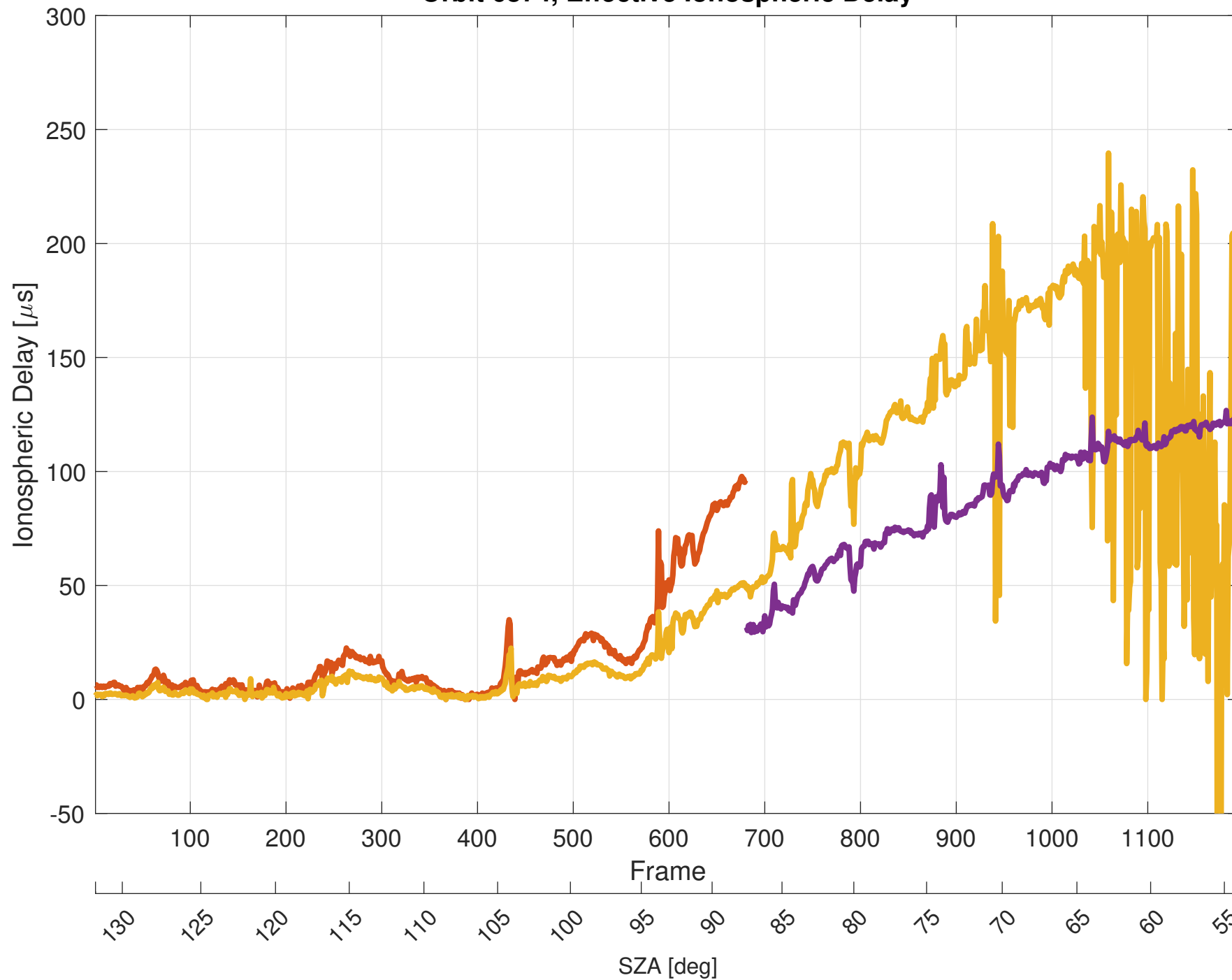
Orbit 6874, Effective Ionospheric Delay
