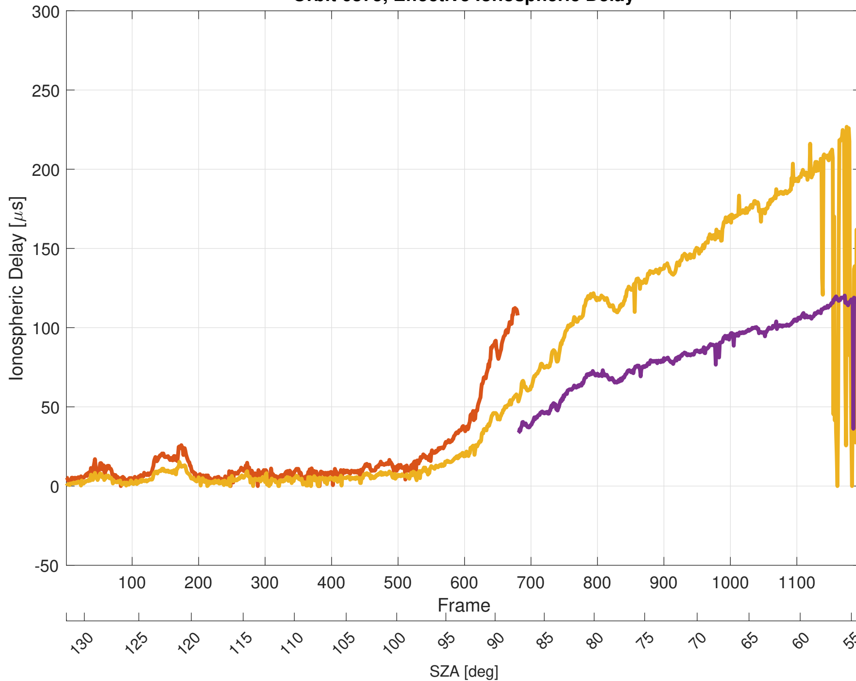
Orbit 6875, Effective Ionospheric Delay
