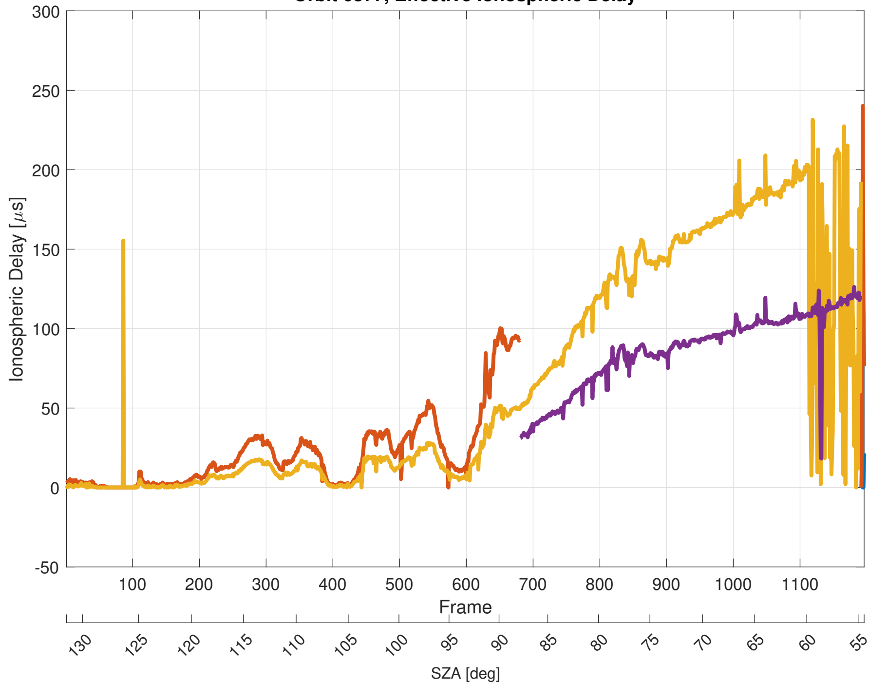
Orbit 6877, Effective Ionospheric Delay
