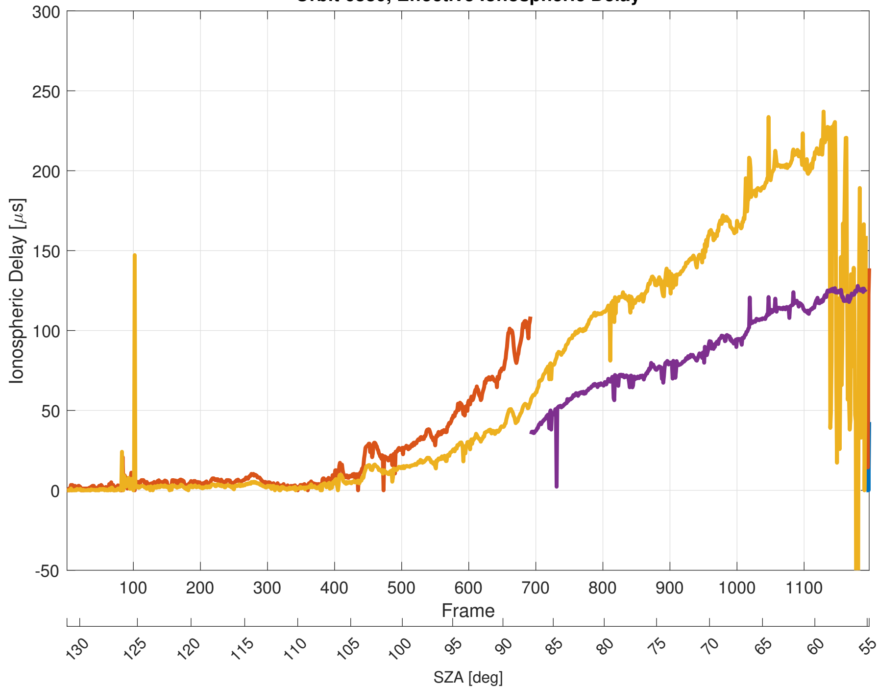
Orbit 6880, Effective Ionospheric Delay
