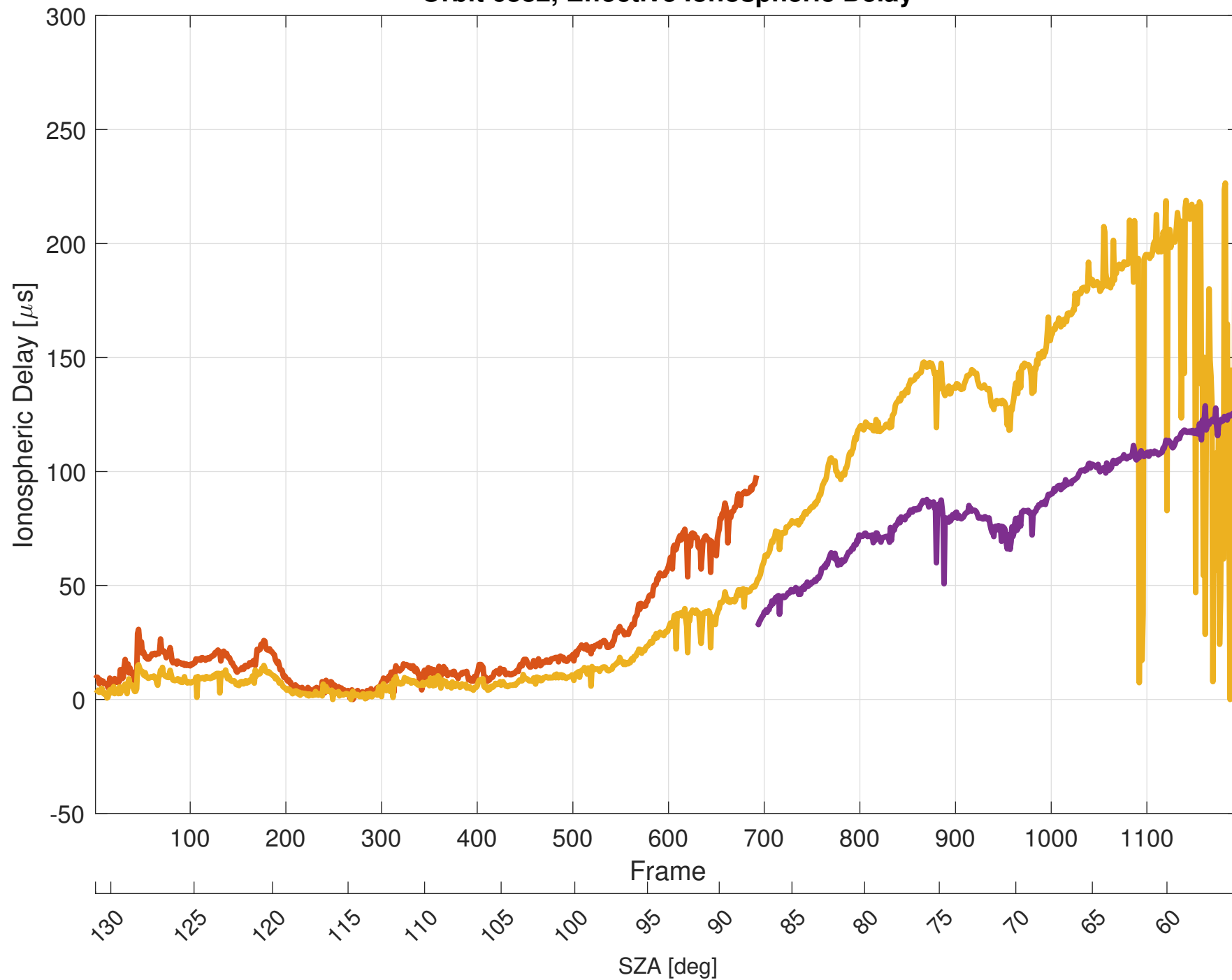
Orbit 6882, Effective Ionospheric Delay
