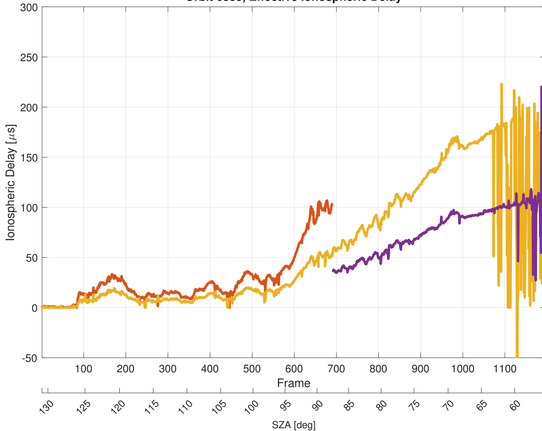
Orbit 6883, Effective Ionospheric Delay
