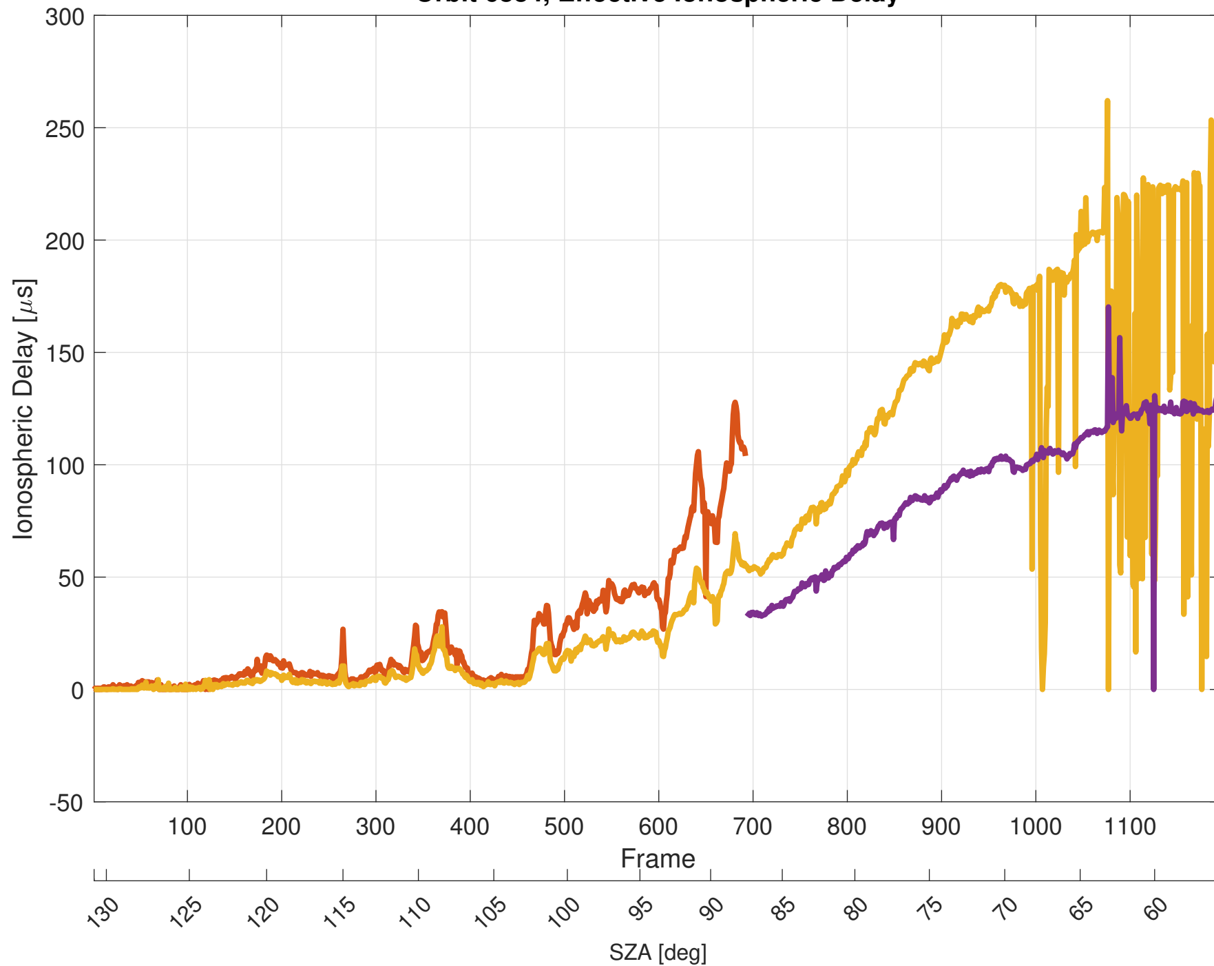
Orbit 6884, Effective Ionospheric Delay
