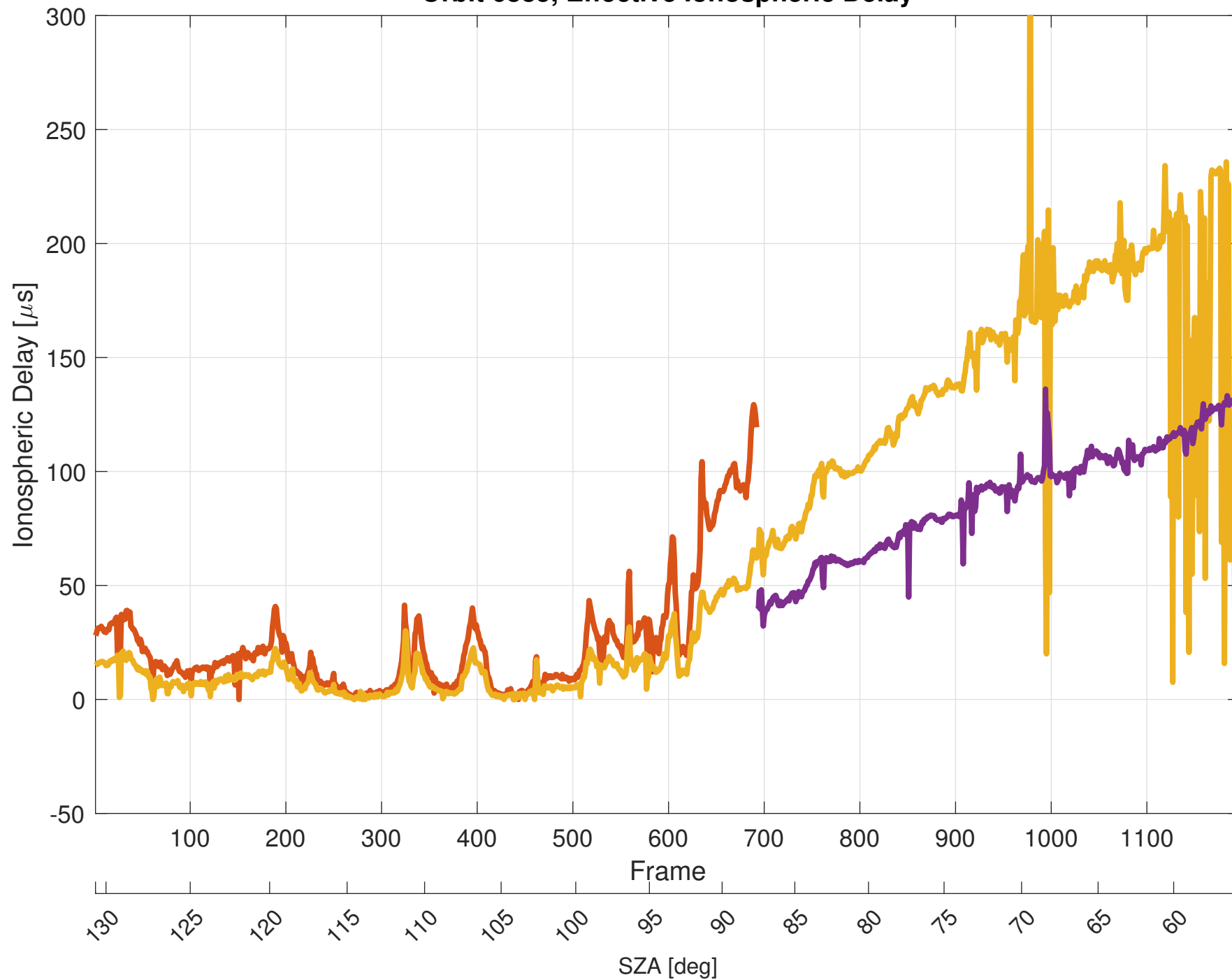
Orbit 6885, Effective Ionospheric Delay
