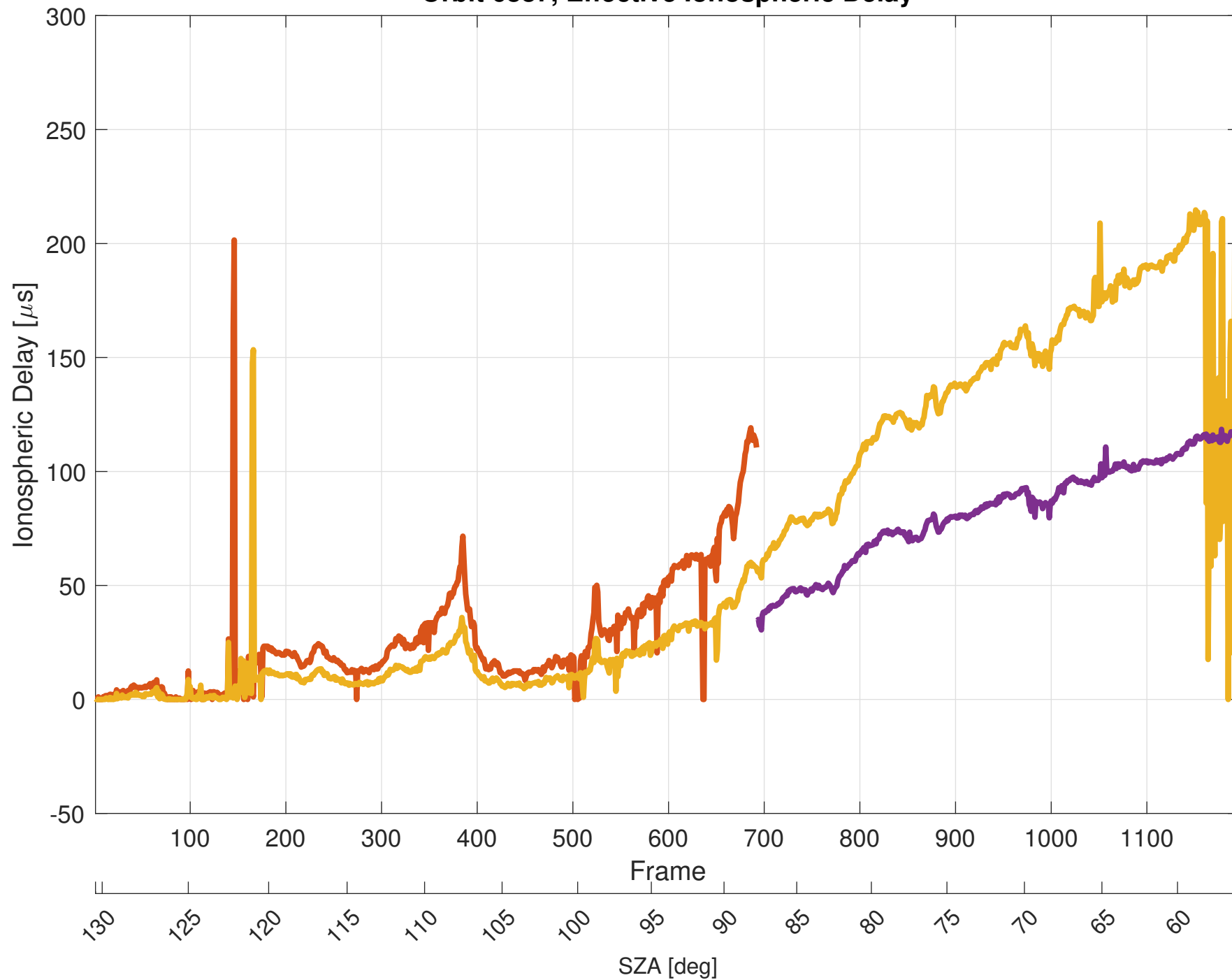
Orbit 6887, Effective Ionospheric Delay
