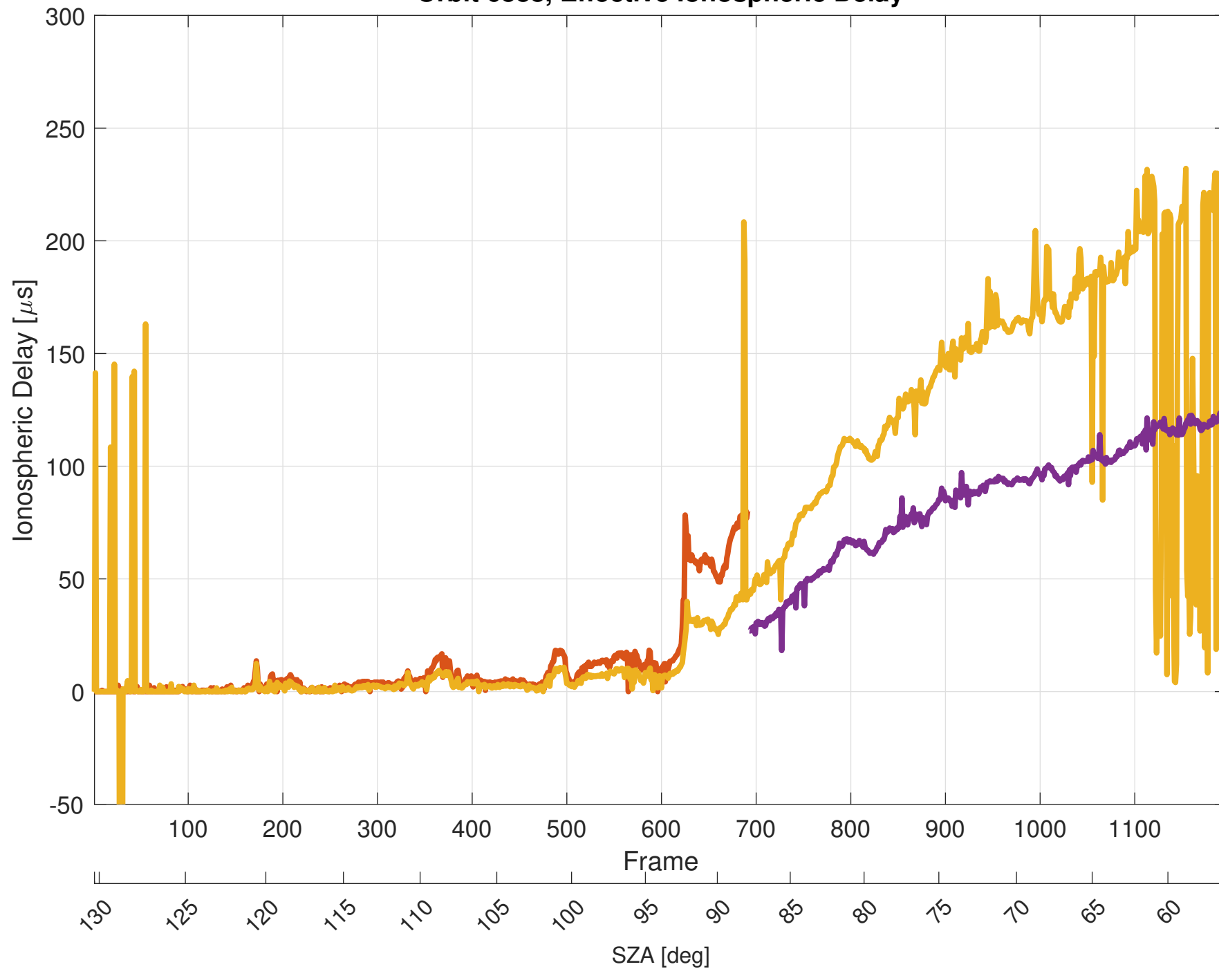
Orbit 6888, Effective Ionospheric Delay
