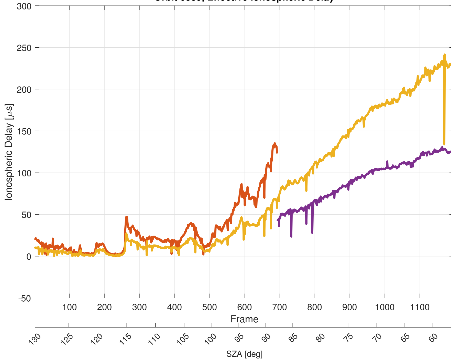
Orbit 6889, Effective Ionospheric Delay
