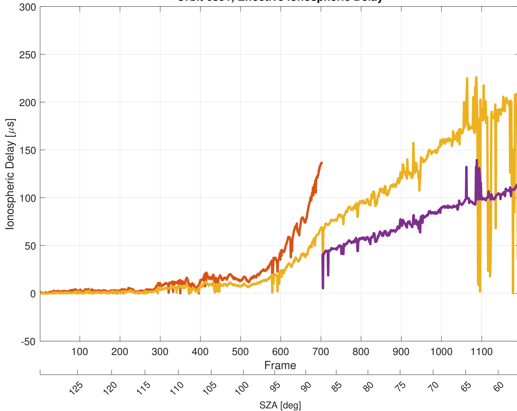
Orbit 6891, Effective Ionospheric Delay
