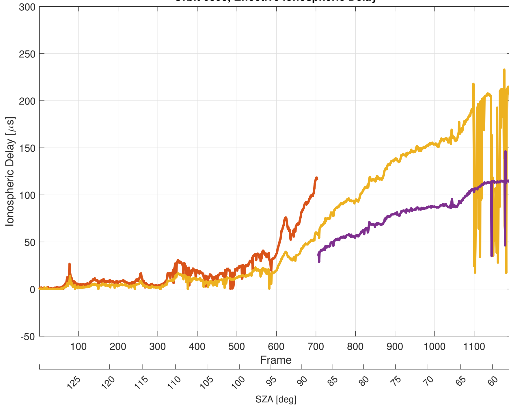
Orbit 6893, Effective Ionospheric Delay
