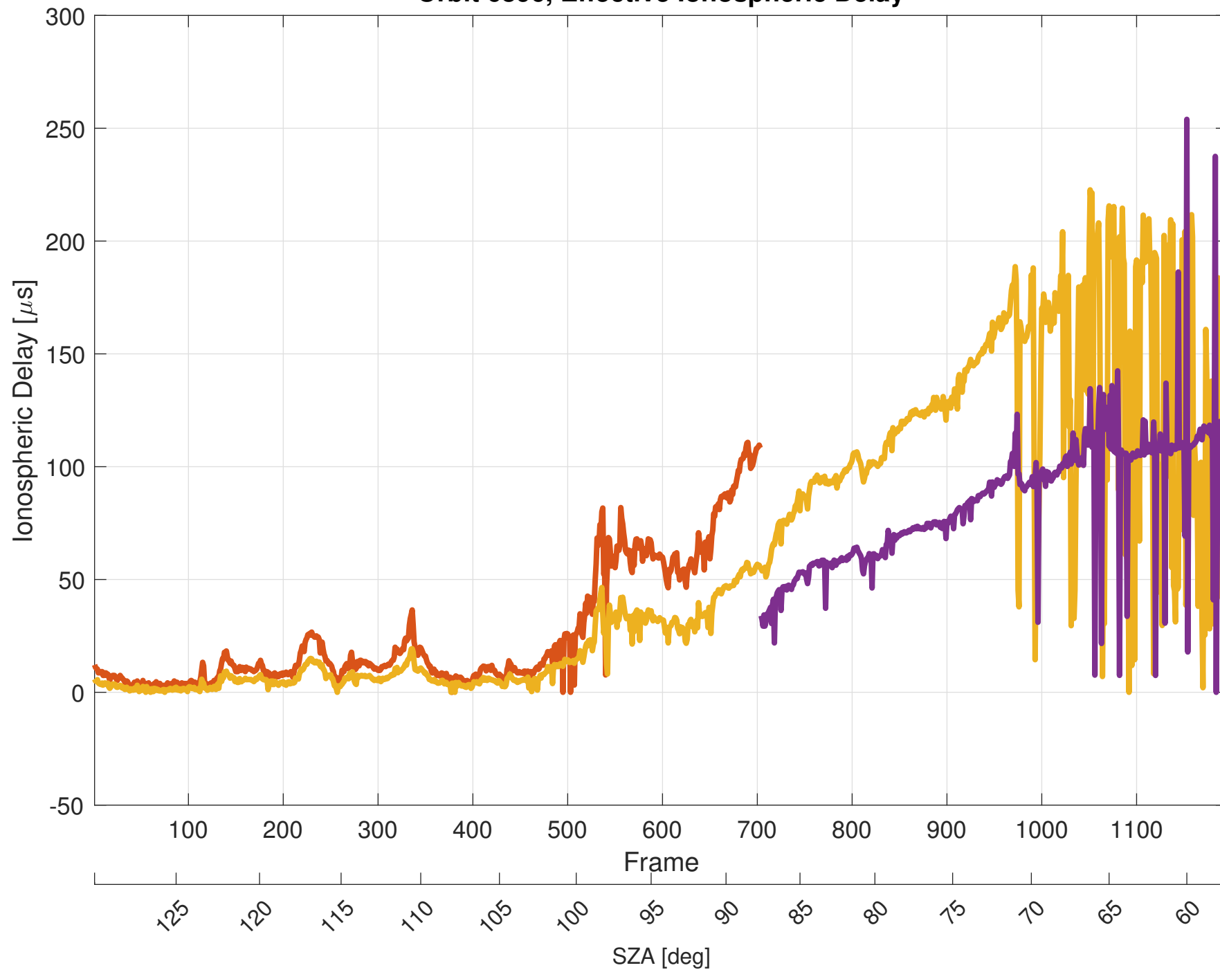
Orbit 6896, Effective Ionospheric Delay
