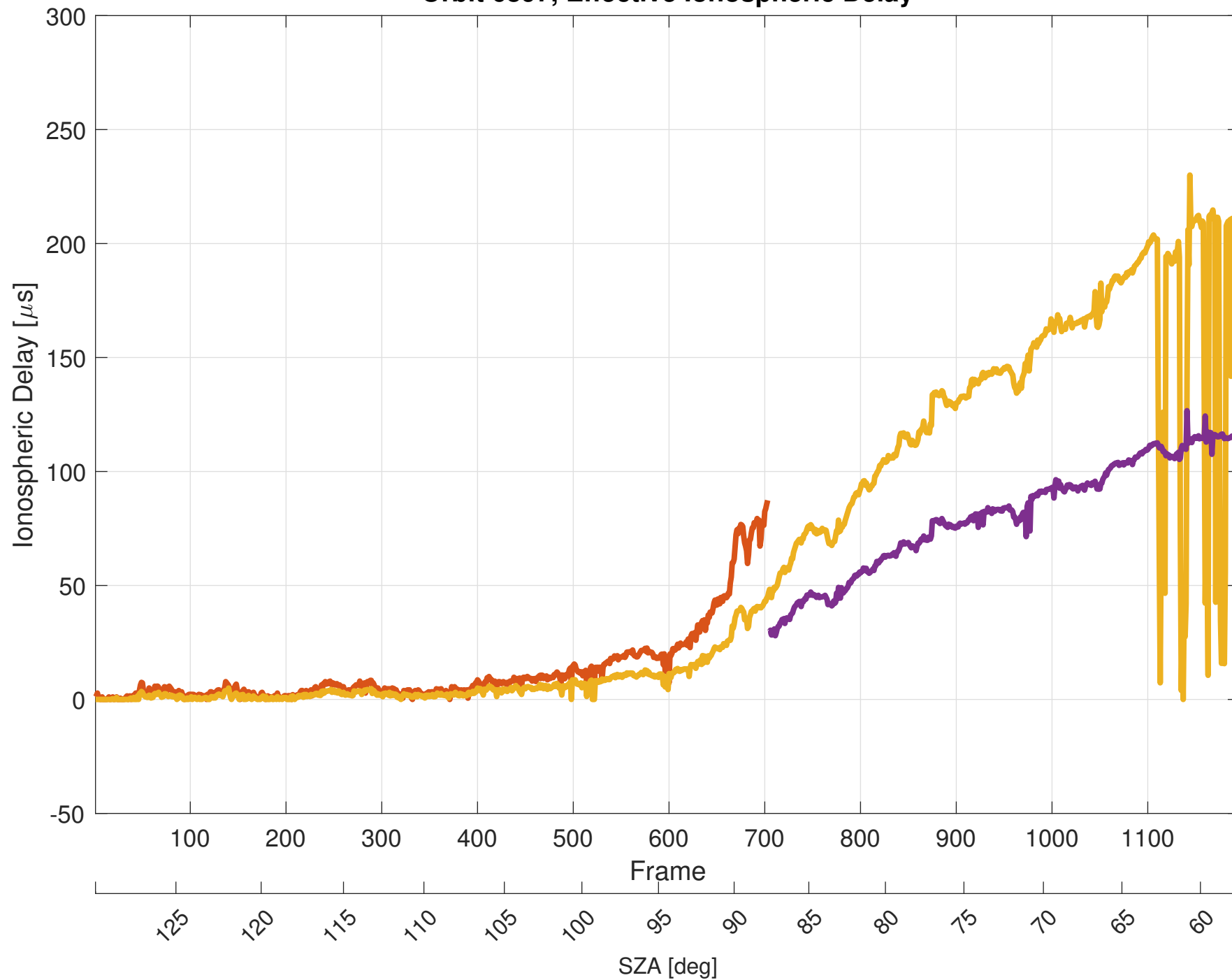
Orbit 6897, Effective Ionospheric Delay
