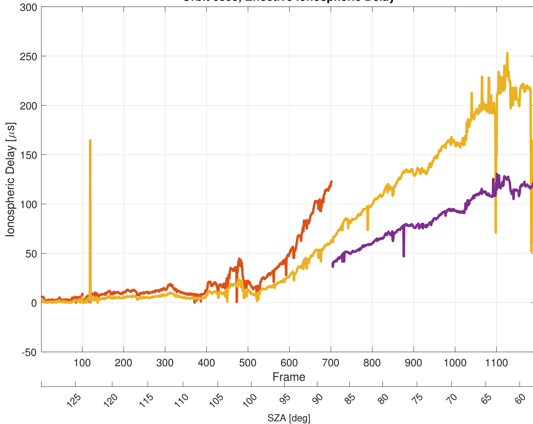
Orbit 6898, Effective Ionospheric Delay
