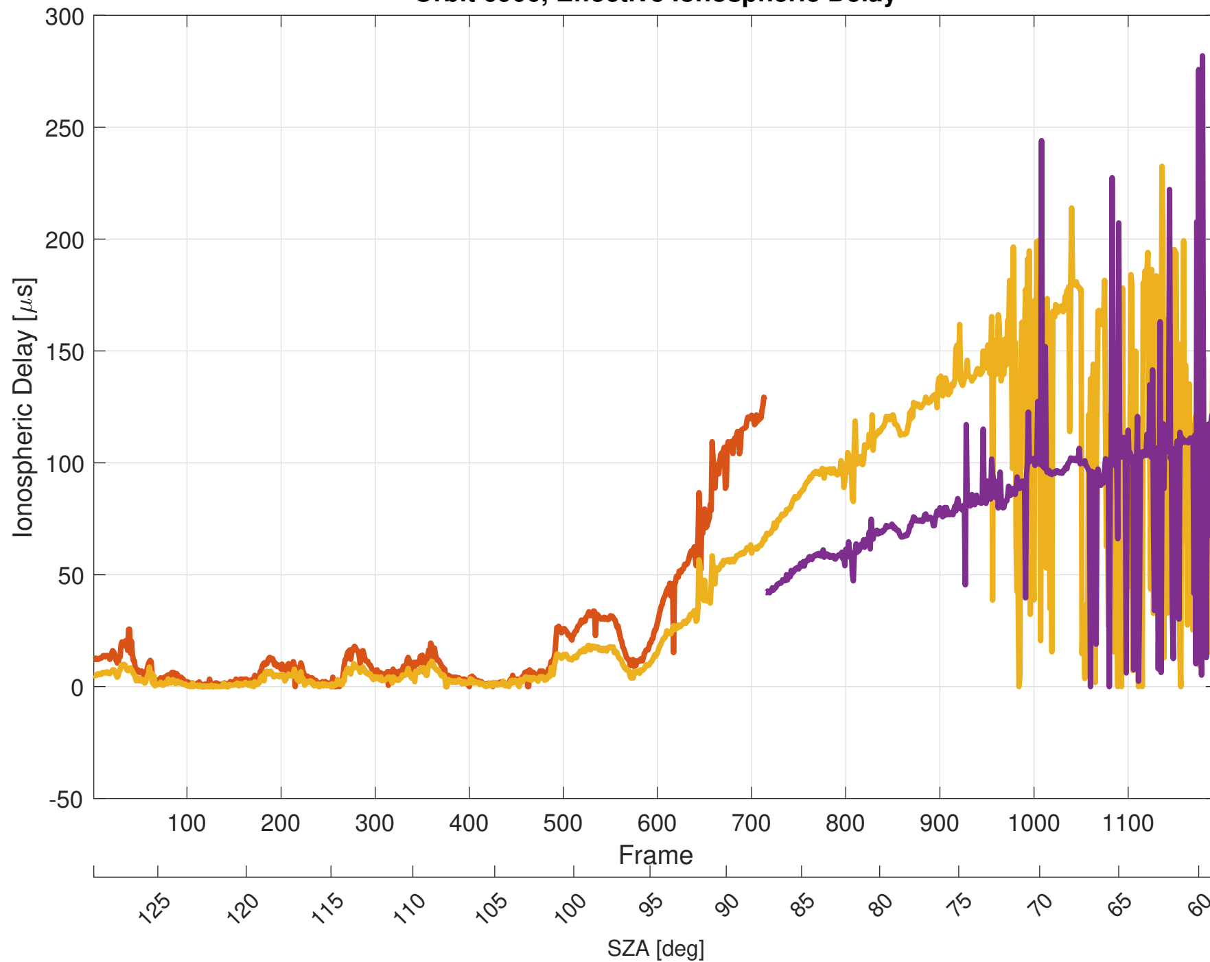
Orbit 6906, Effective Ionospheric Delay
