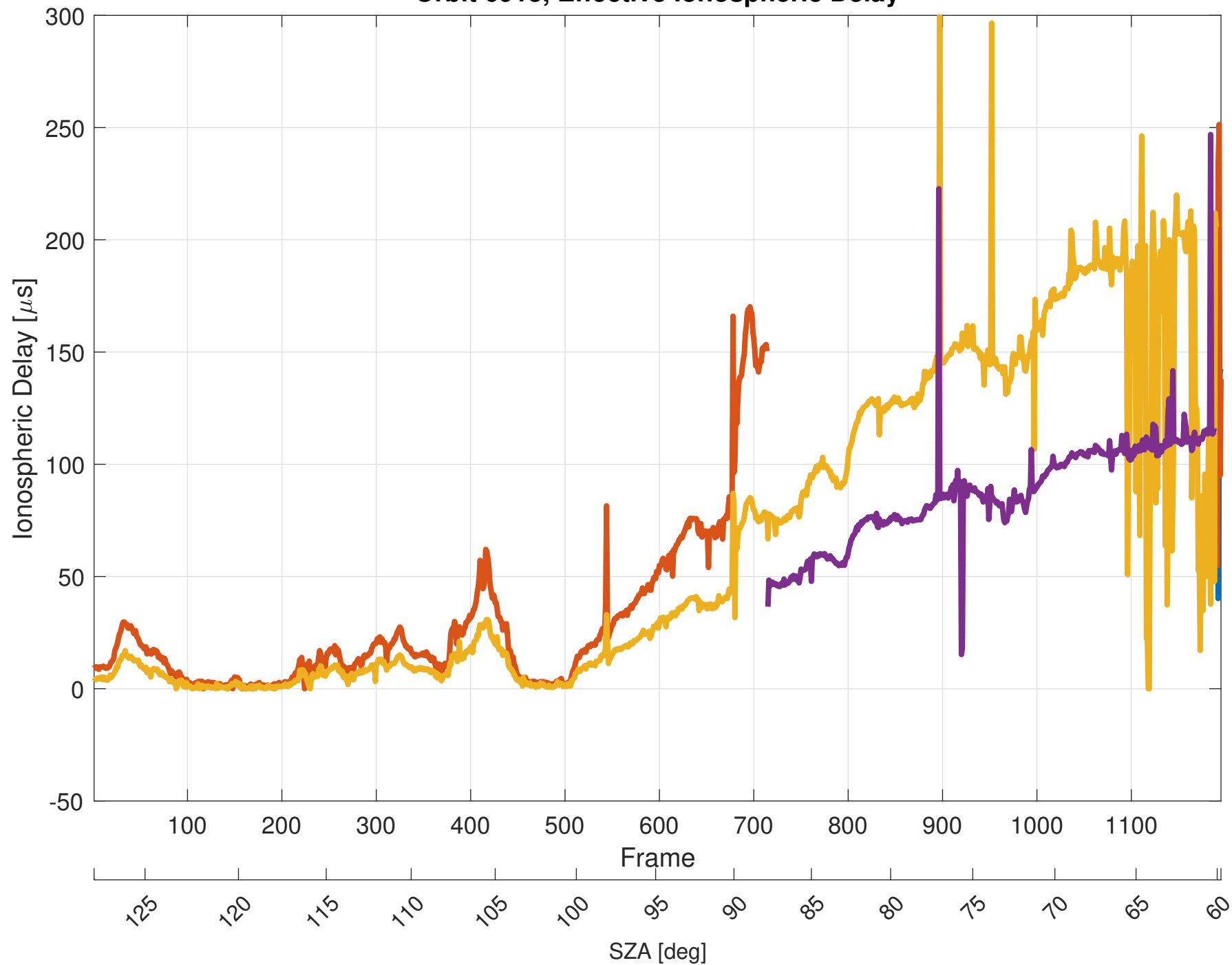
Orbit 6913, Effective Ionospheric Delay
