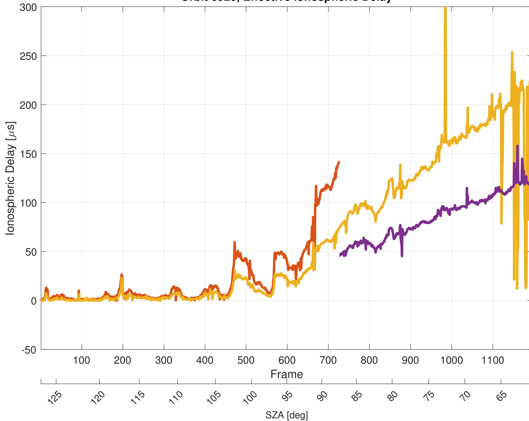
Orbit 6920, Effective Ionospheric Delay
