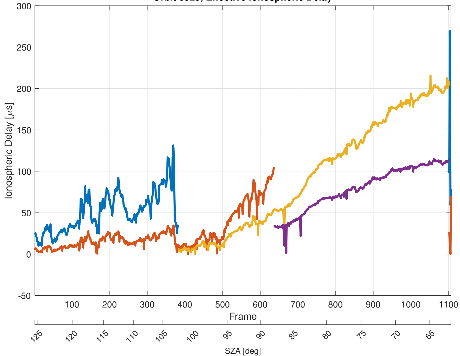
Orbit 6929, Effective Ionospheric Delay
