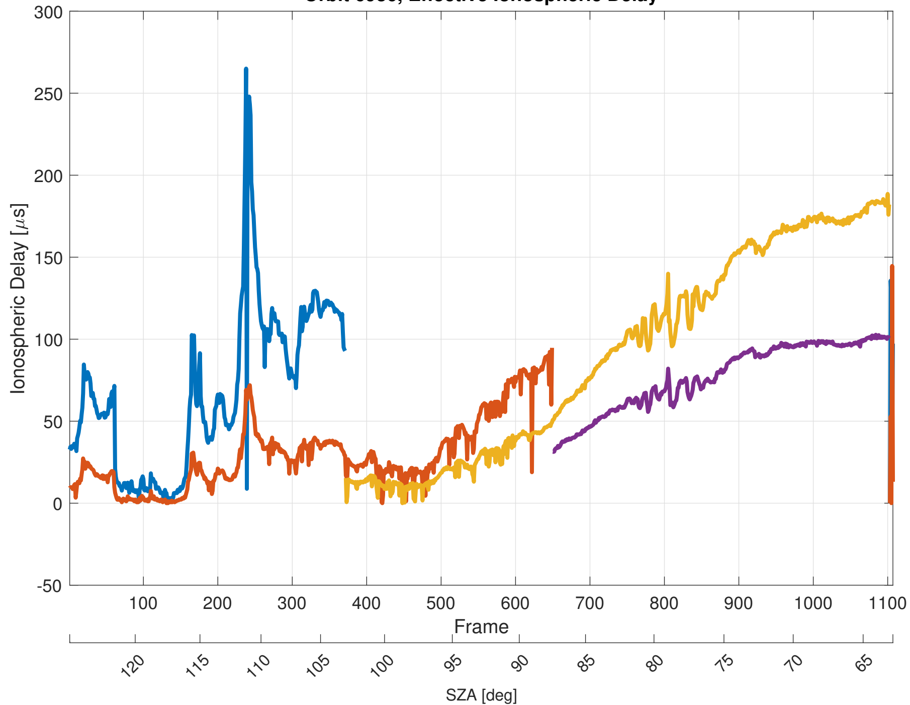
Orbit 6936, Effective Ionospheric Delay
