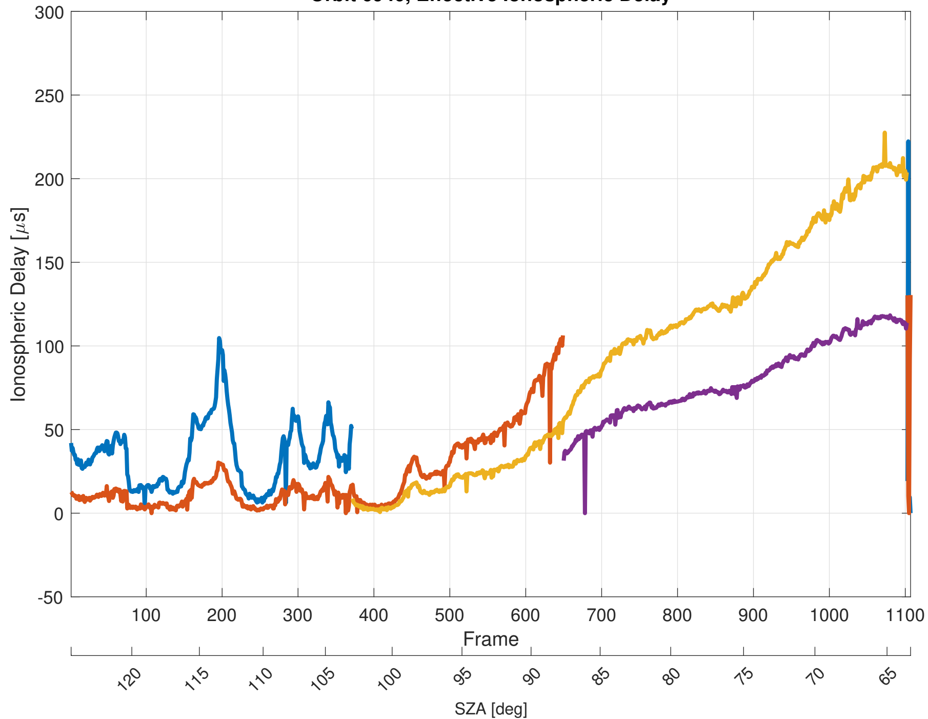
Orbit 6940, Effective Ionospheric Delay
