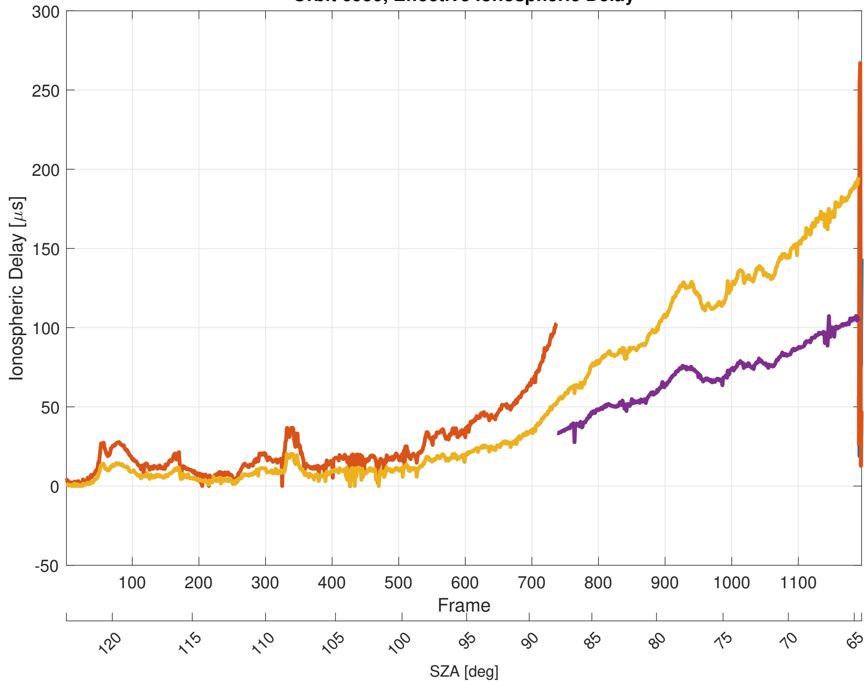
Orbit 6950, Effective Ionospheric Delay
