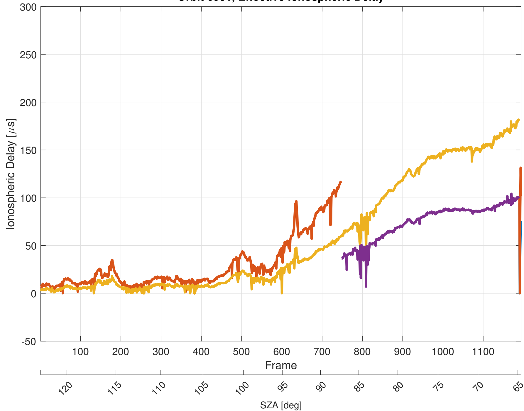
Orbit 6951, Effective Ionospheric Delay
