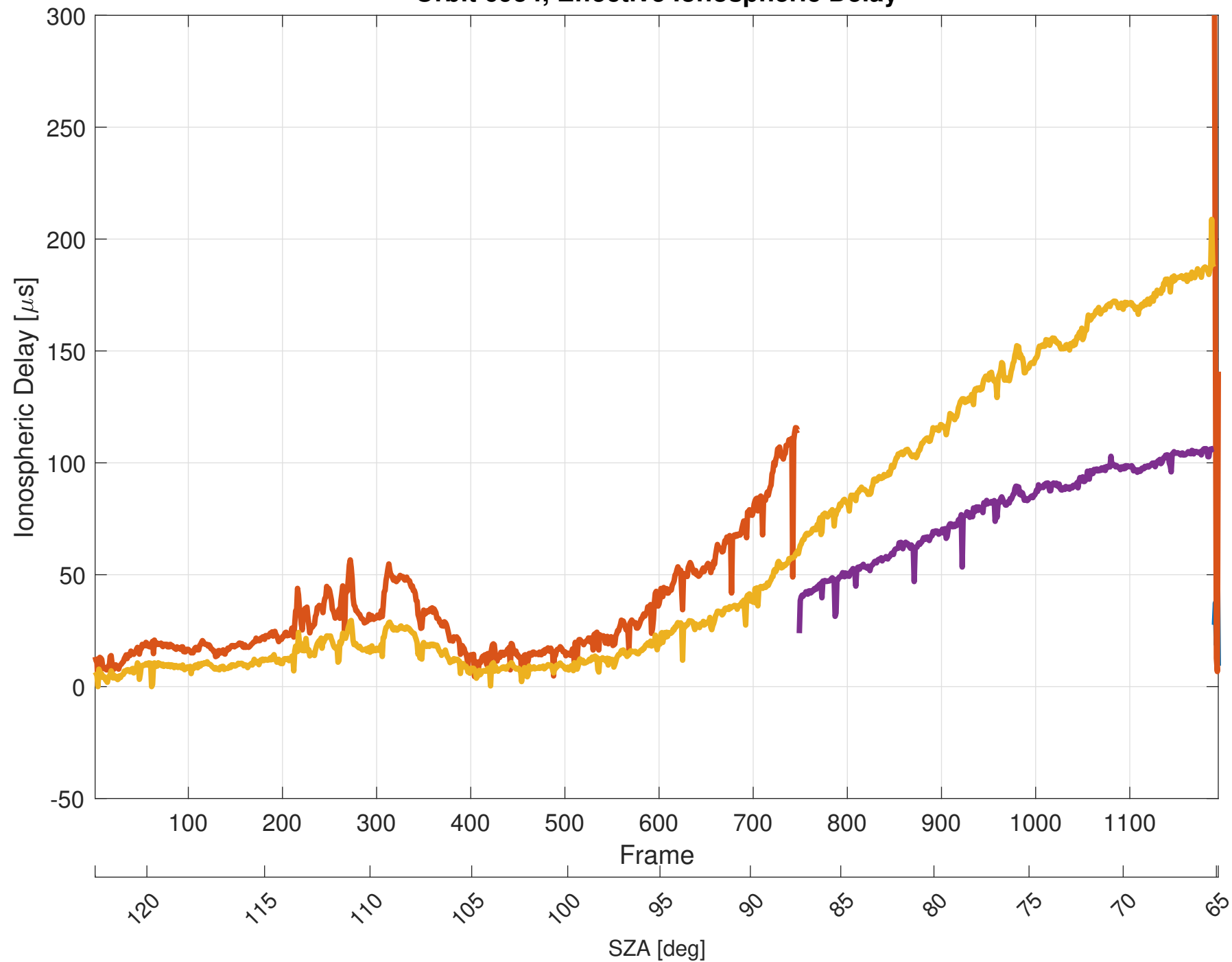
Orbit 6954, Effective Ionospheric Delay
