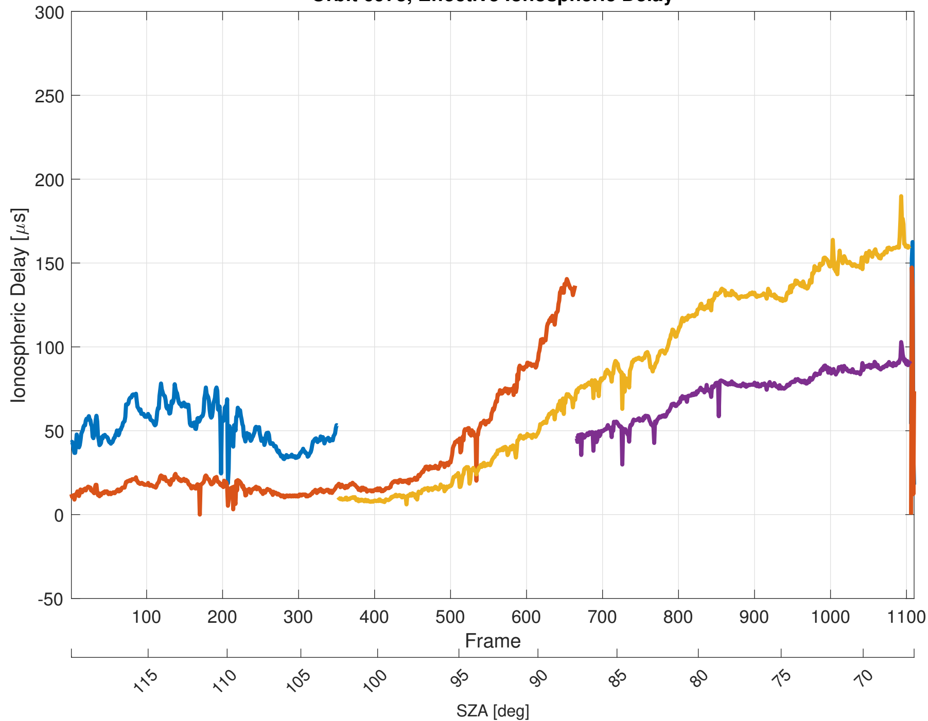
Orbit 6973, Effective Ionospheric Delay
