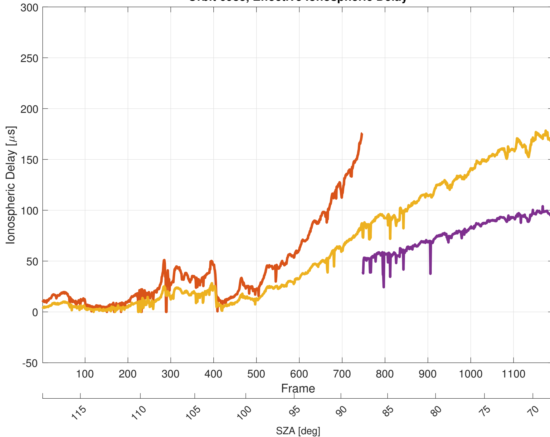
Orbit 6983, Effective Ionospheric Delay
