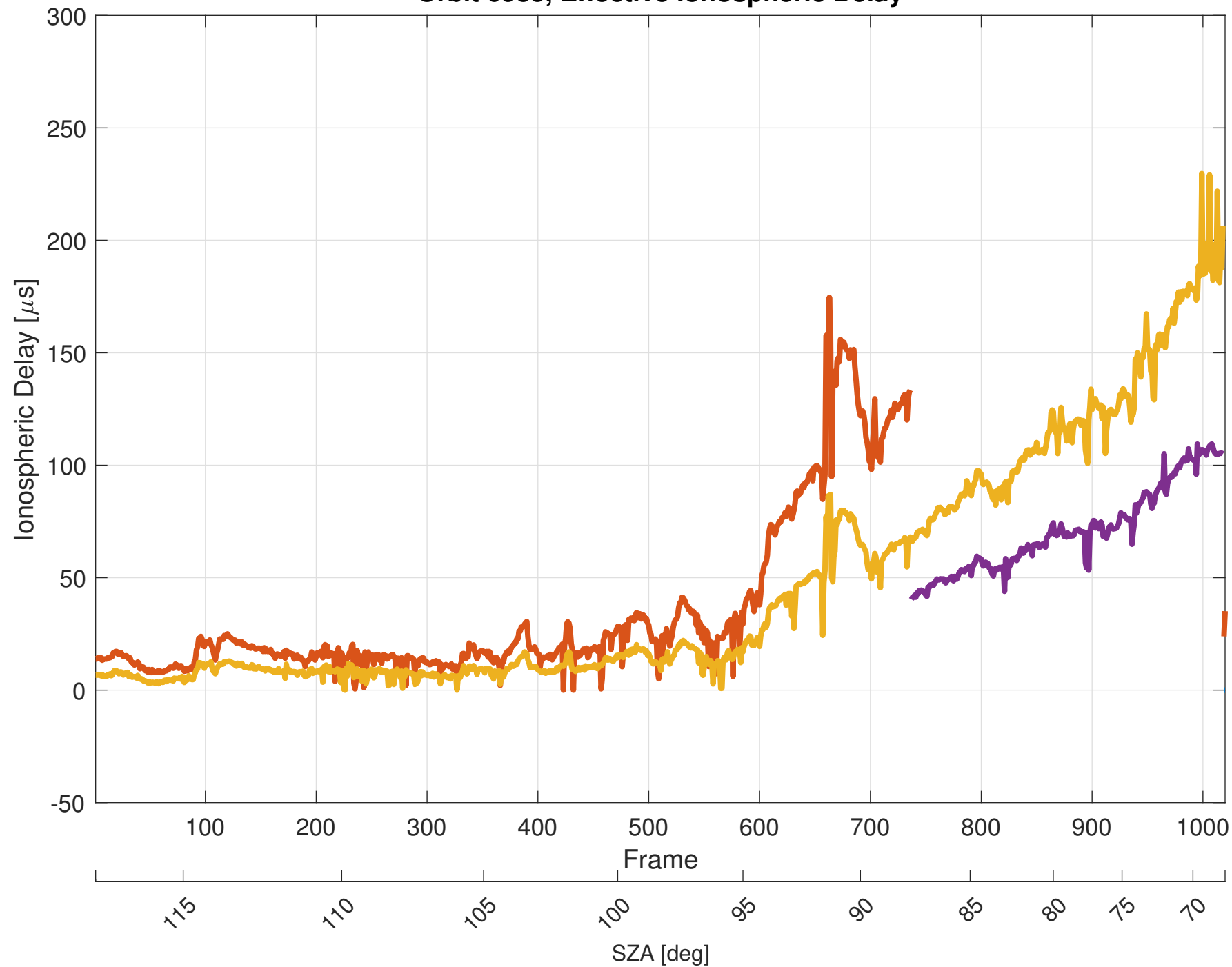
Orbit 6985, Effective Ionospheric Delay
