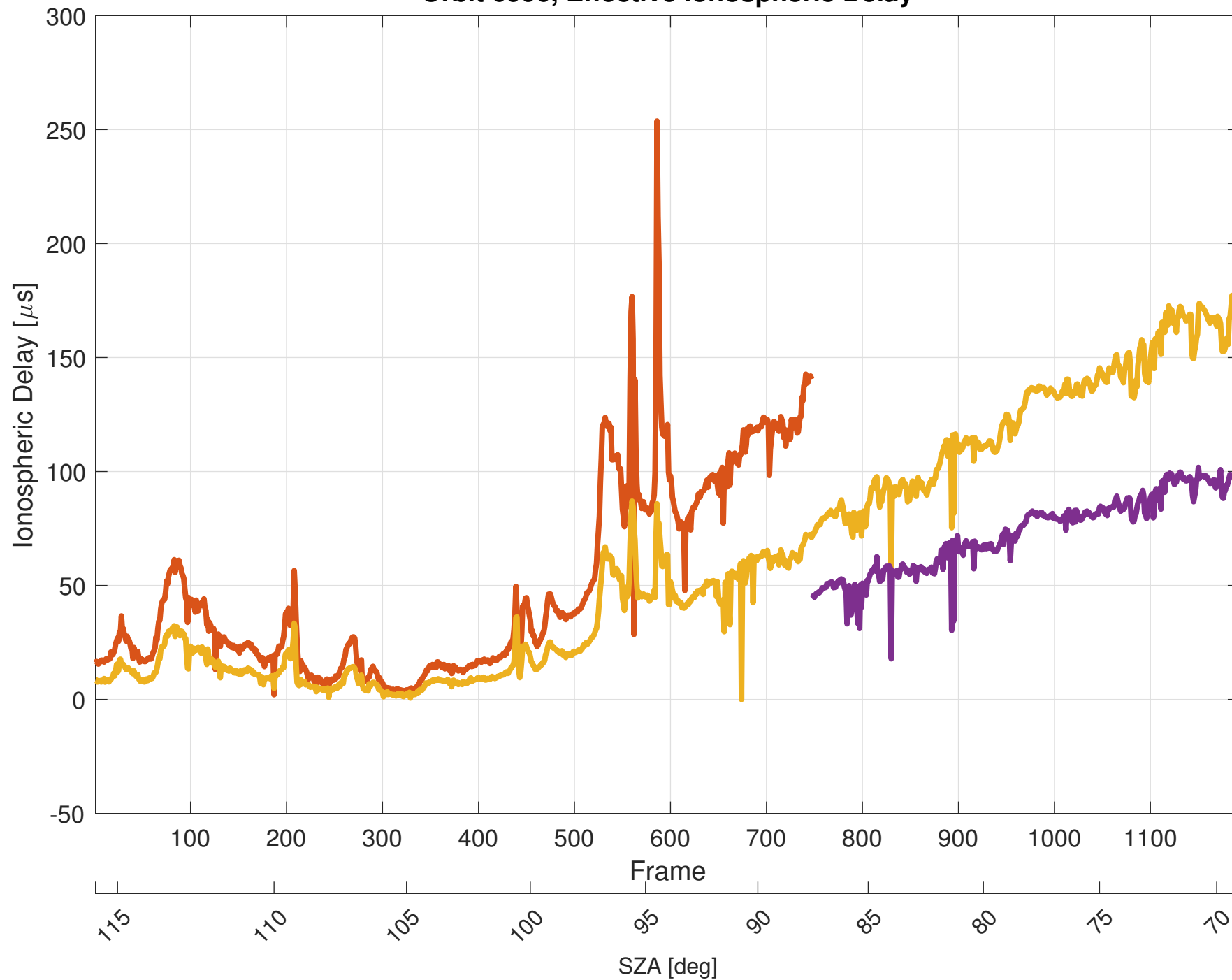
Orbit 6996, Effective Ionospheric Delay
