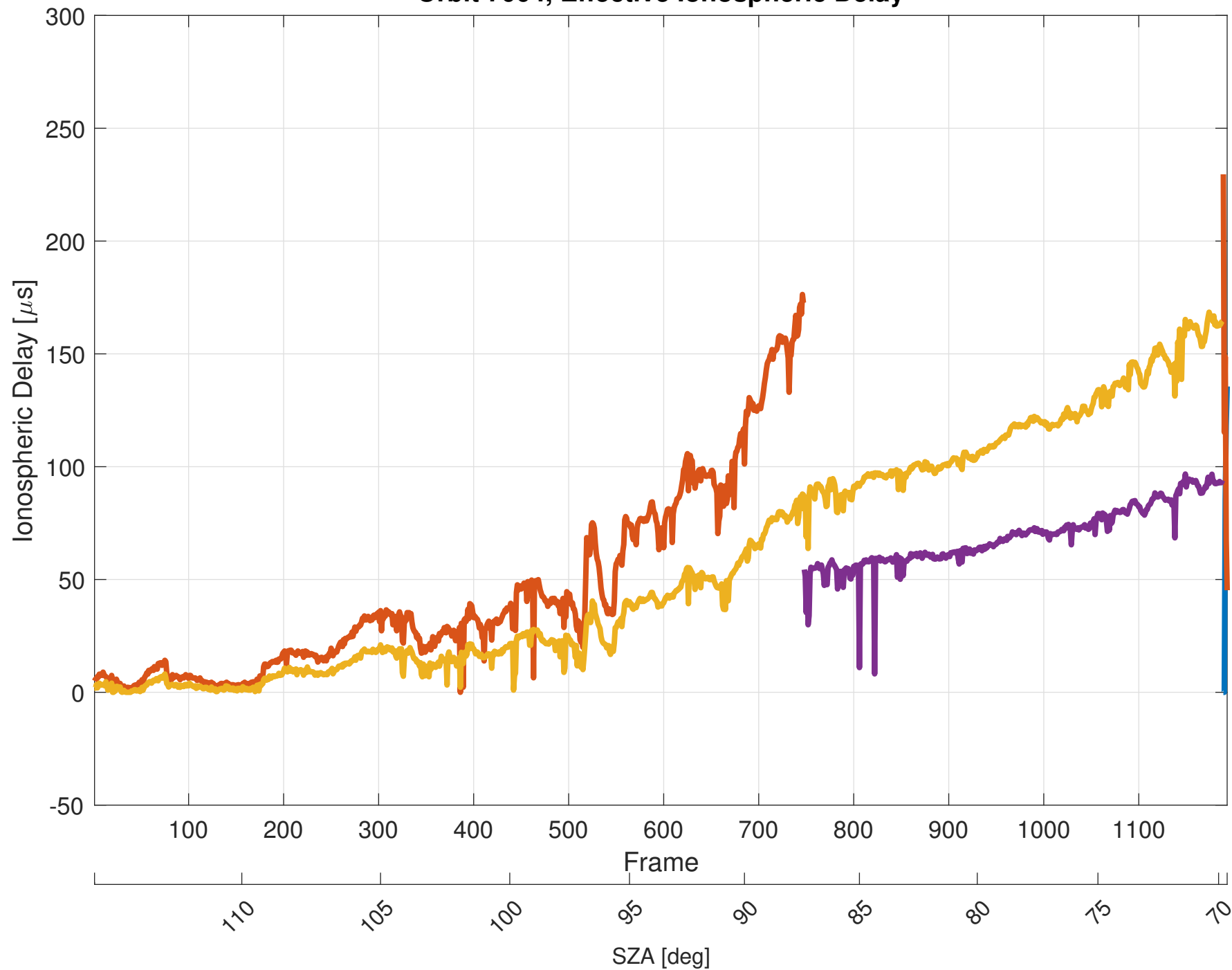
Orbit 7004, Effective Ionospheric Delay
