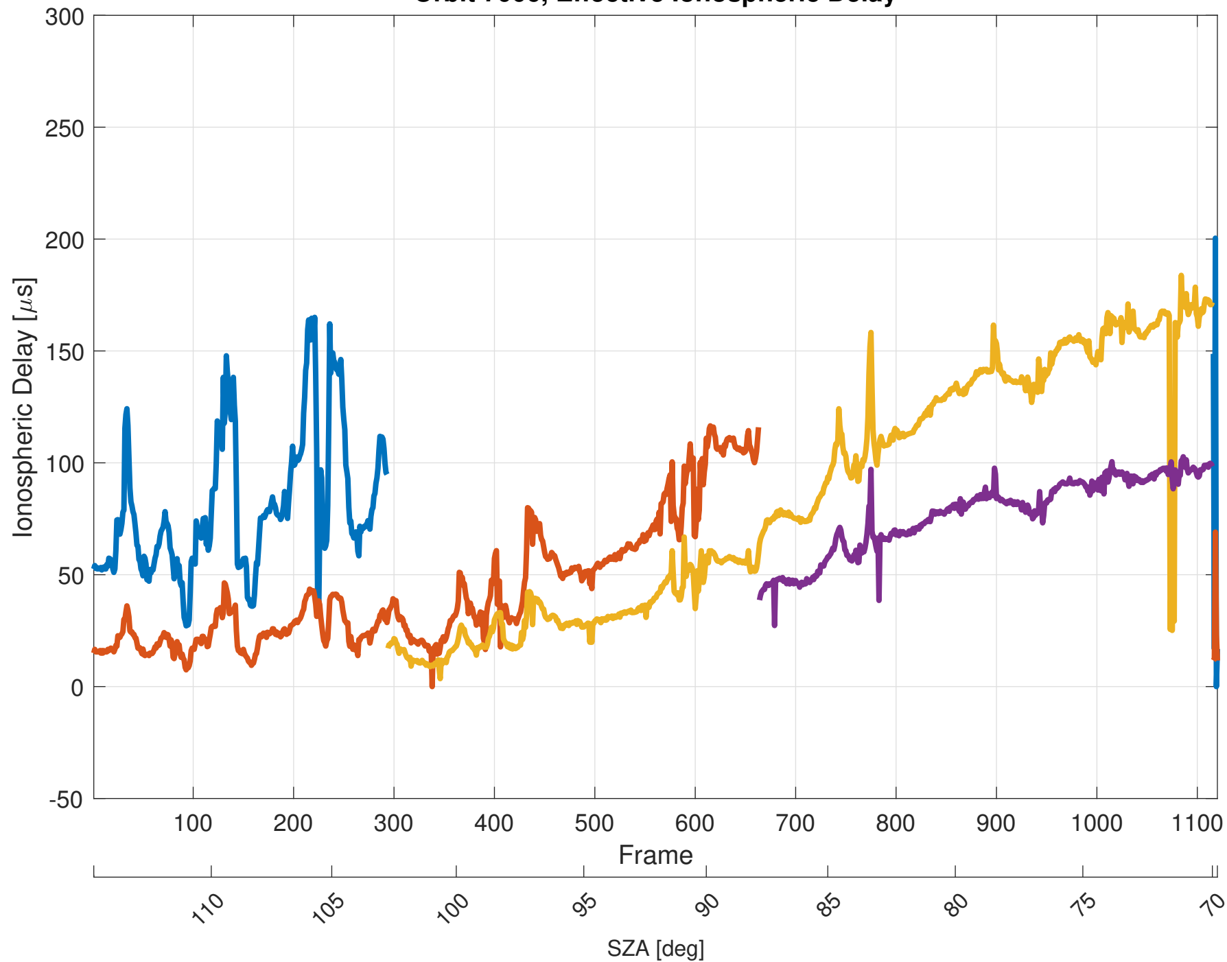
Orbit 7006, Effective Ionospheric Delay
