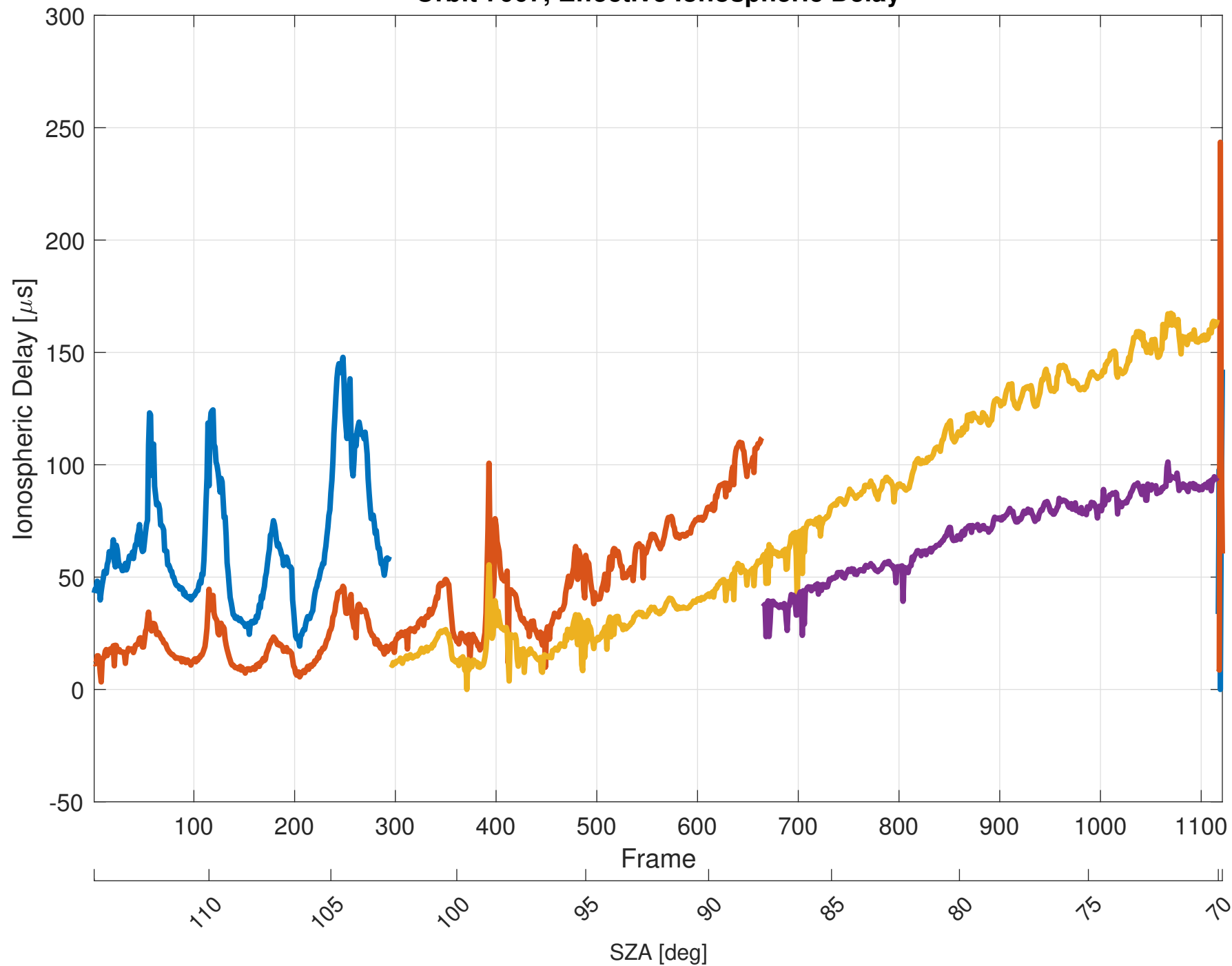
Orbit 7007, Effective Ionospheric Delay
