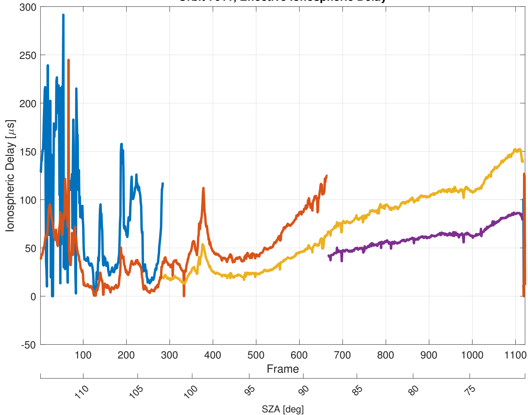
Orbit 7011, Effective Ionospheric Delay
