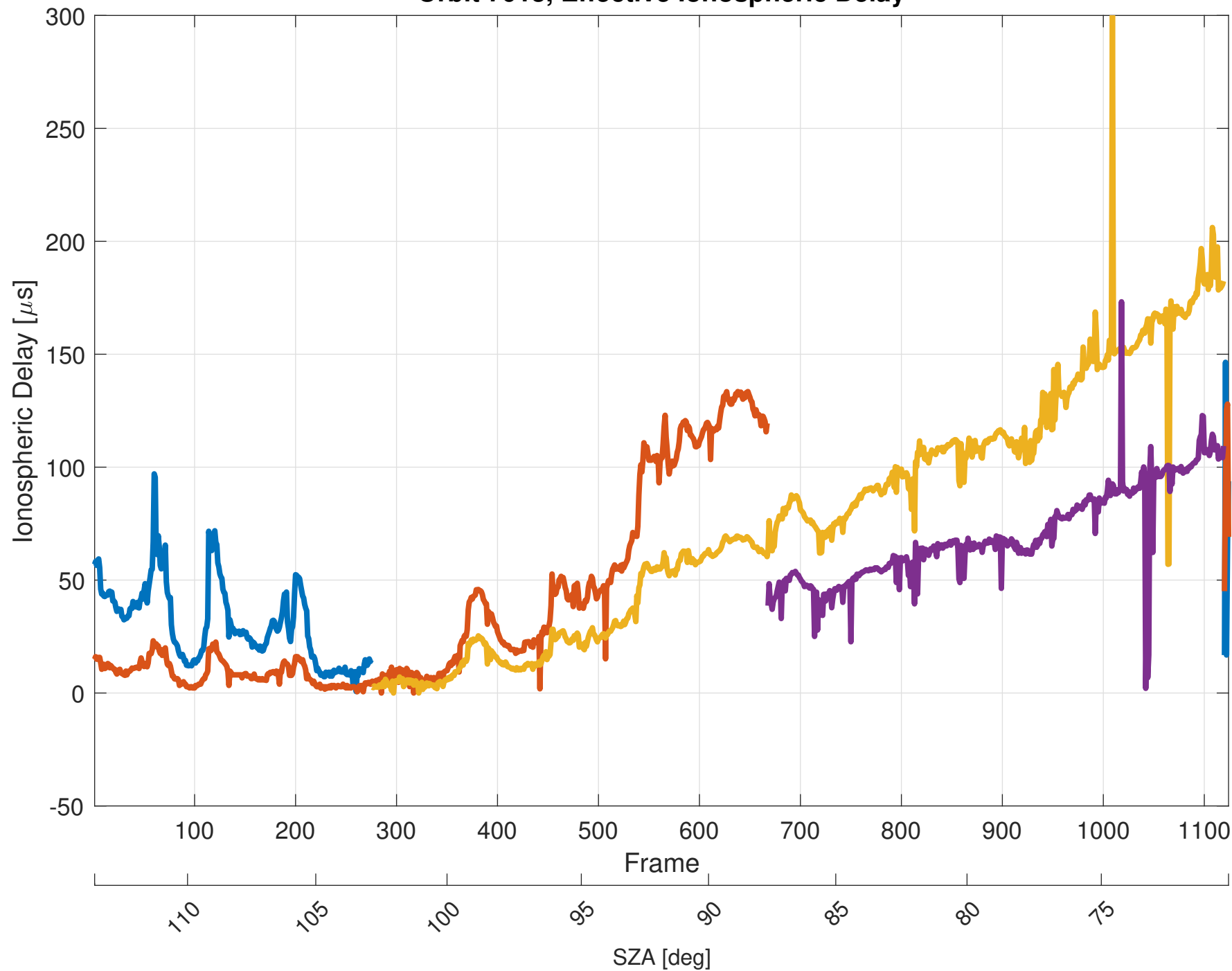
Orbit 7013, Effective Ionospheric Delay
