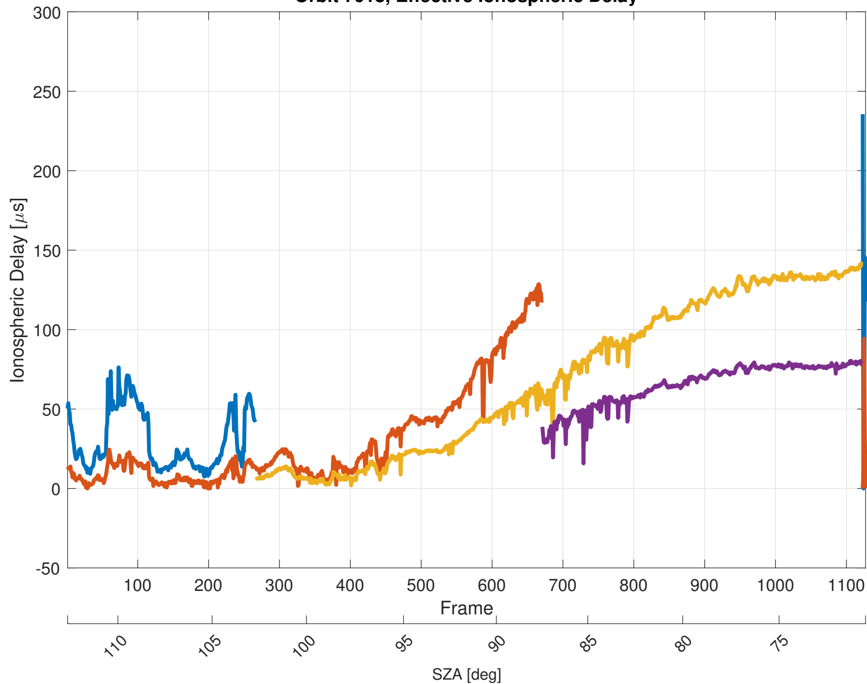
Orbit 7018, Effective Ionospheric Delay
