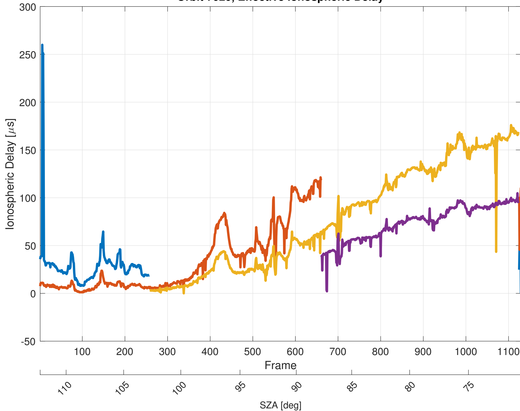
Orbit 7020, Effective Ionospheric Delay
