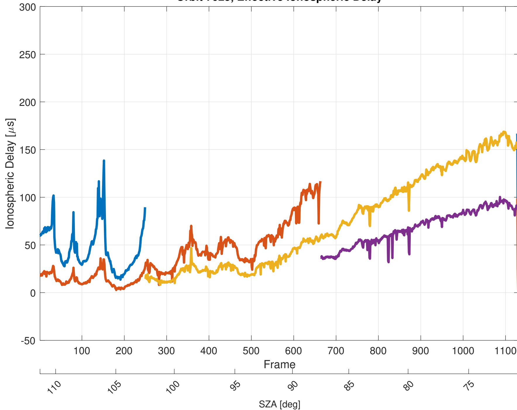
Orbit 7025, Effective Ionospheric Delay
