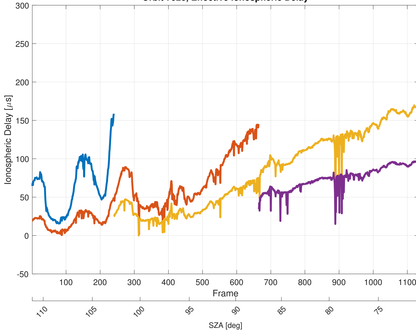
Orbit 7026, Effective Ionospheric Delay
