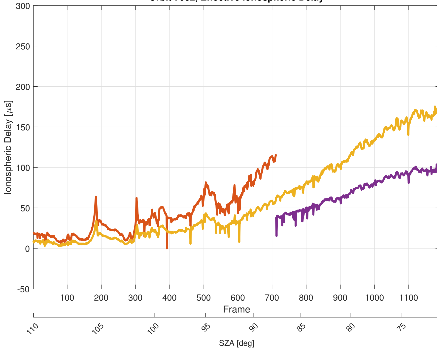
Orbit 7032, Effective Ionospheric Delay
