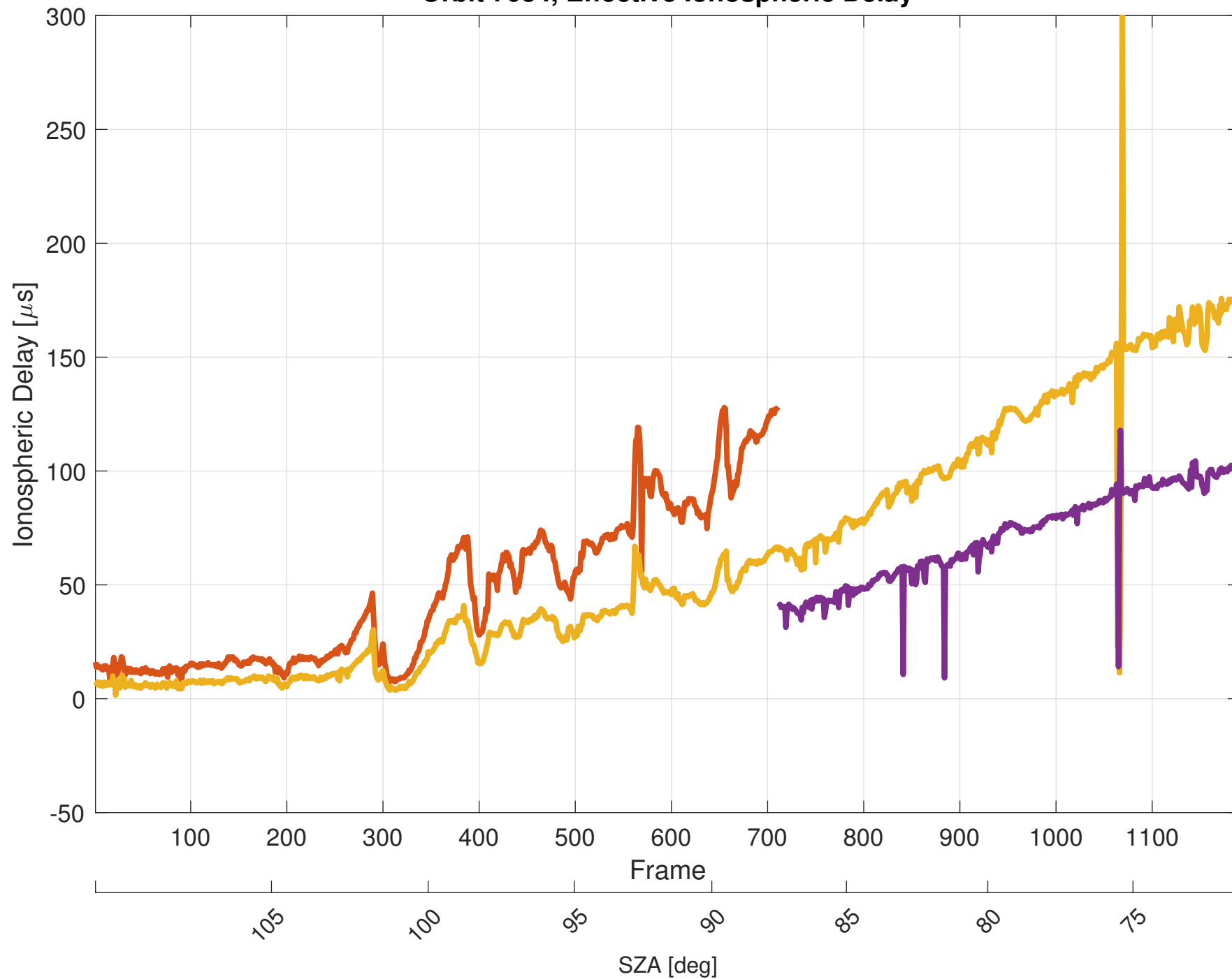
Orbit 7034, Effective Ionospheric Delay
