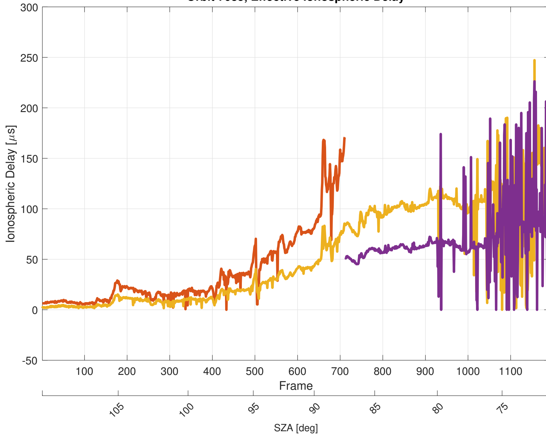
Orbit 7035, Effective Ionospheric Delay
