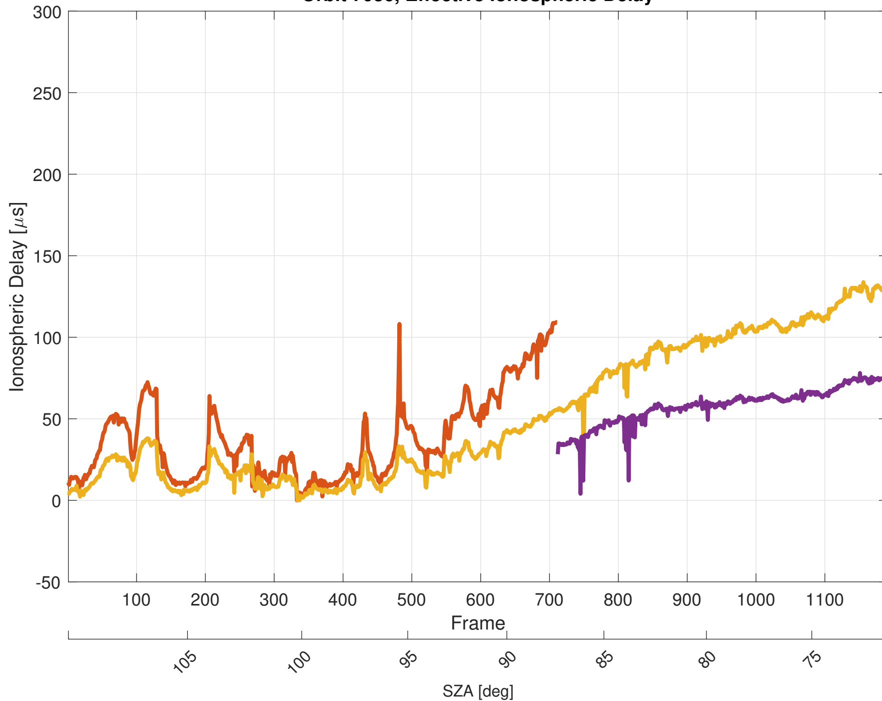
Orbit 7036, Effective Ionospheric Delay
