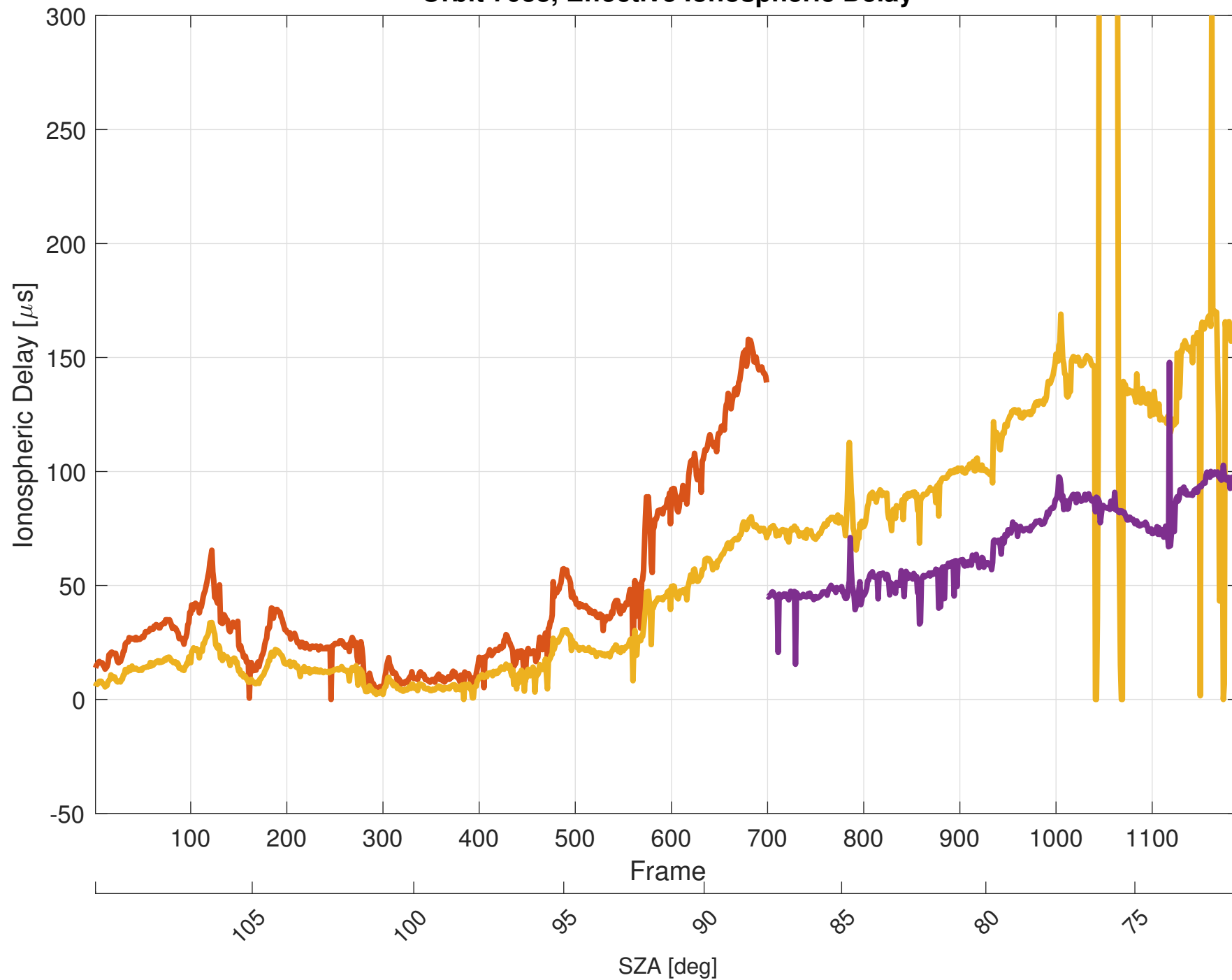
Orbit 7038, Effective Ionospheric Delay
