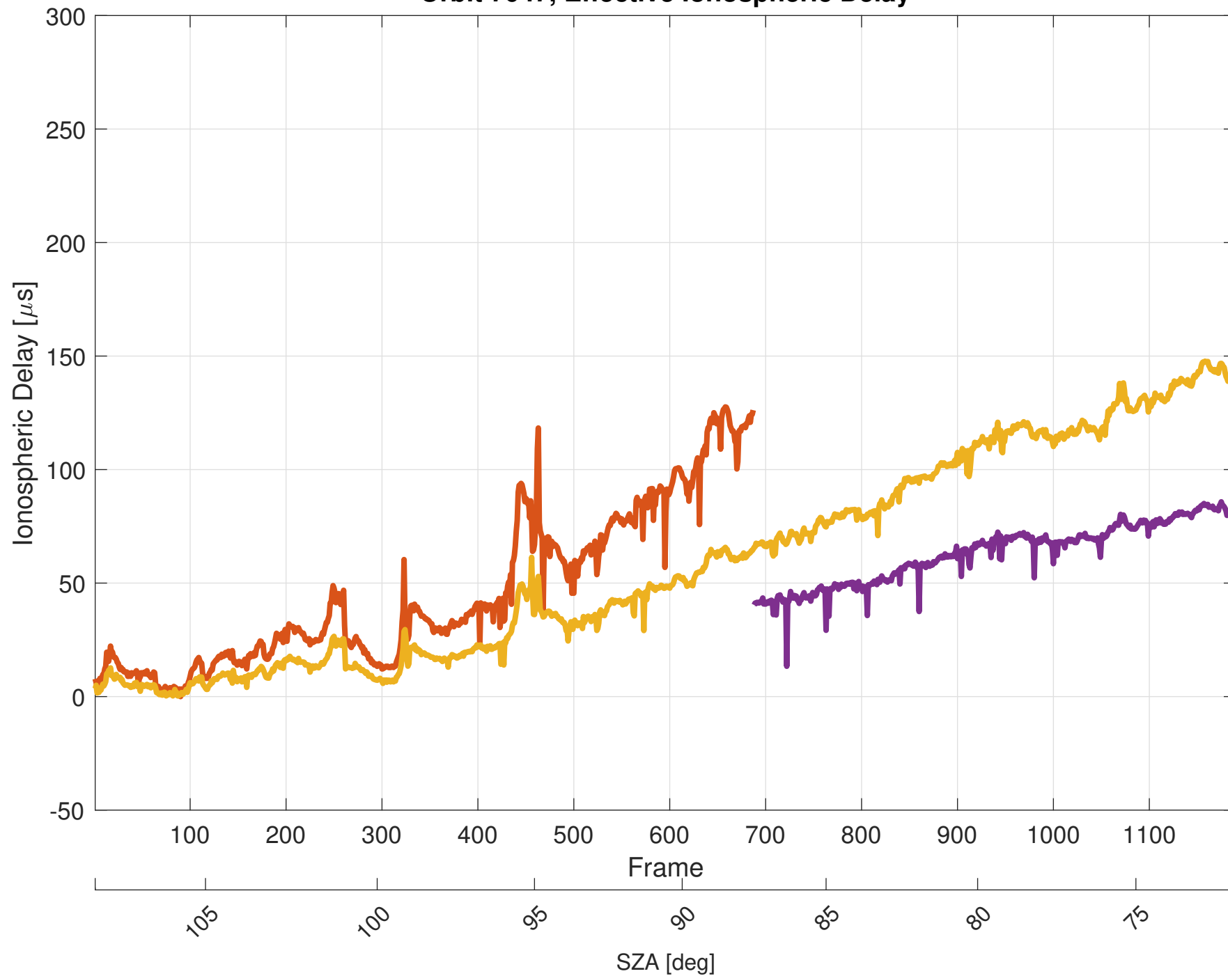
Orbit 7047, Effective Ionospheric Delay
